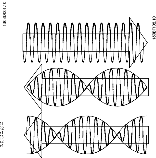
Illustration 5.6 Resolversignaler
