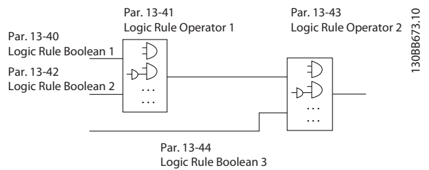
Illustration 2.7 Logiske regler
