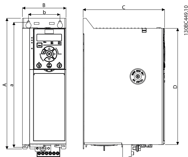
Illustration 4.10 Dimensions
