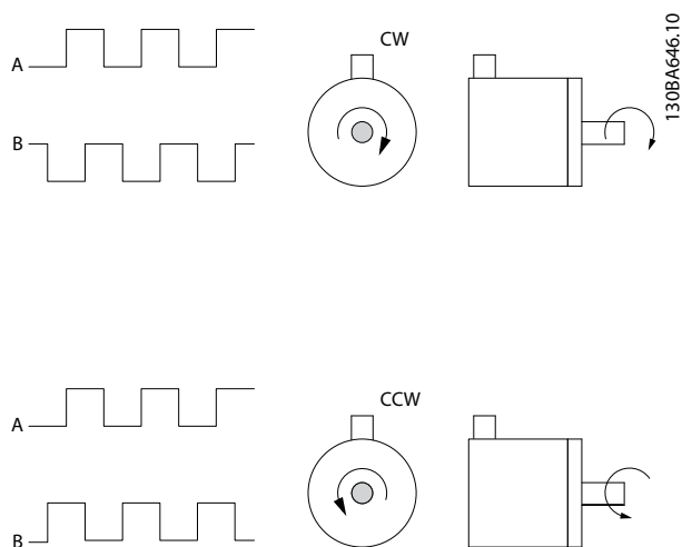
Illustration 6.3 24 V Incremental Encoder, Maximum Cable Length 5 m (16.4 ft)
