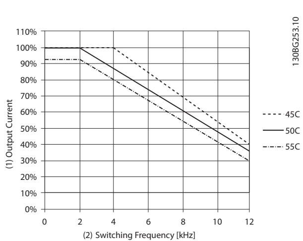
Illustration 4.8 J6 Derating Curve
