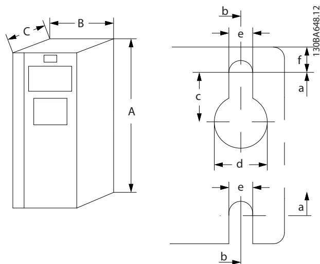
Illustration 4.11 Top and Bottom Mounting Holes J1–J5
