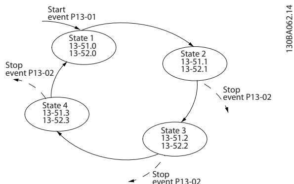
Illustration 2.37 Sequence with 3 Events/Actions
