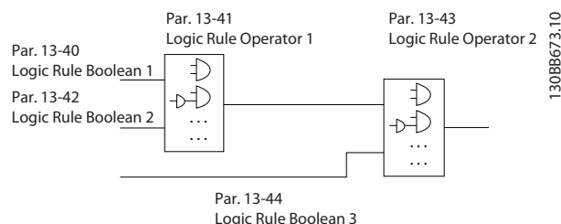
Illustration 2.39 Logic Rules
