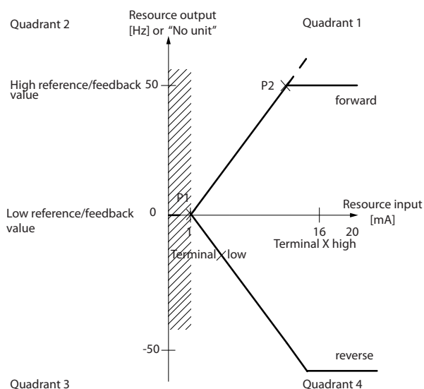
Illustration 2.21 Size of Dead Band
