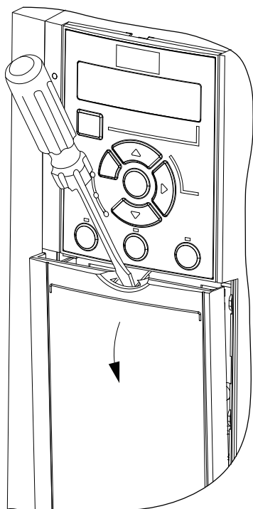
Illustration 2.6 Control Wiring Access for Enclosure Sizes J1-J7
