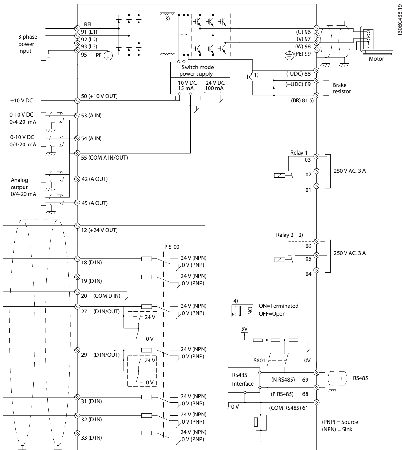
Illustration 2.1 Basic Wiring Schematic Drawing
