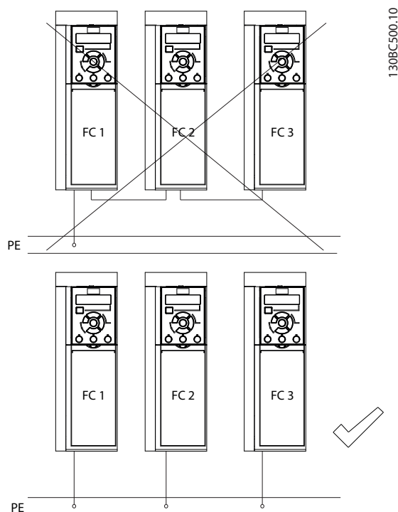
Illustration 2.3 Grounding Principle
