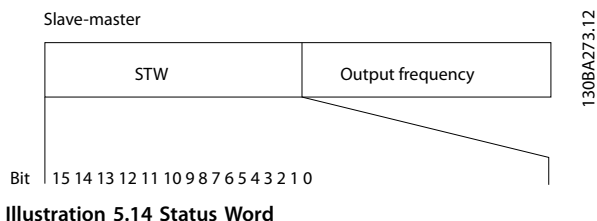
Illustration 5.14 Status Word
