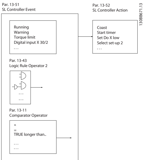
Illustration 2.36 Associated Action
