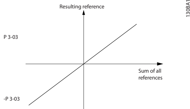
Illustration 2.18 Sum of All References When Reference Range is Set to 1
