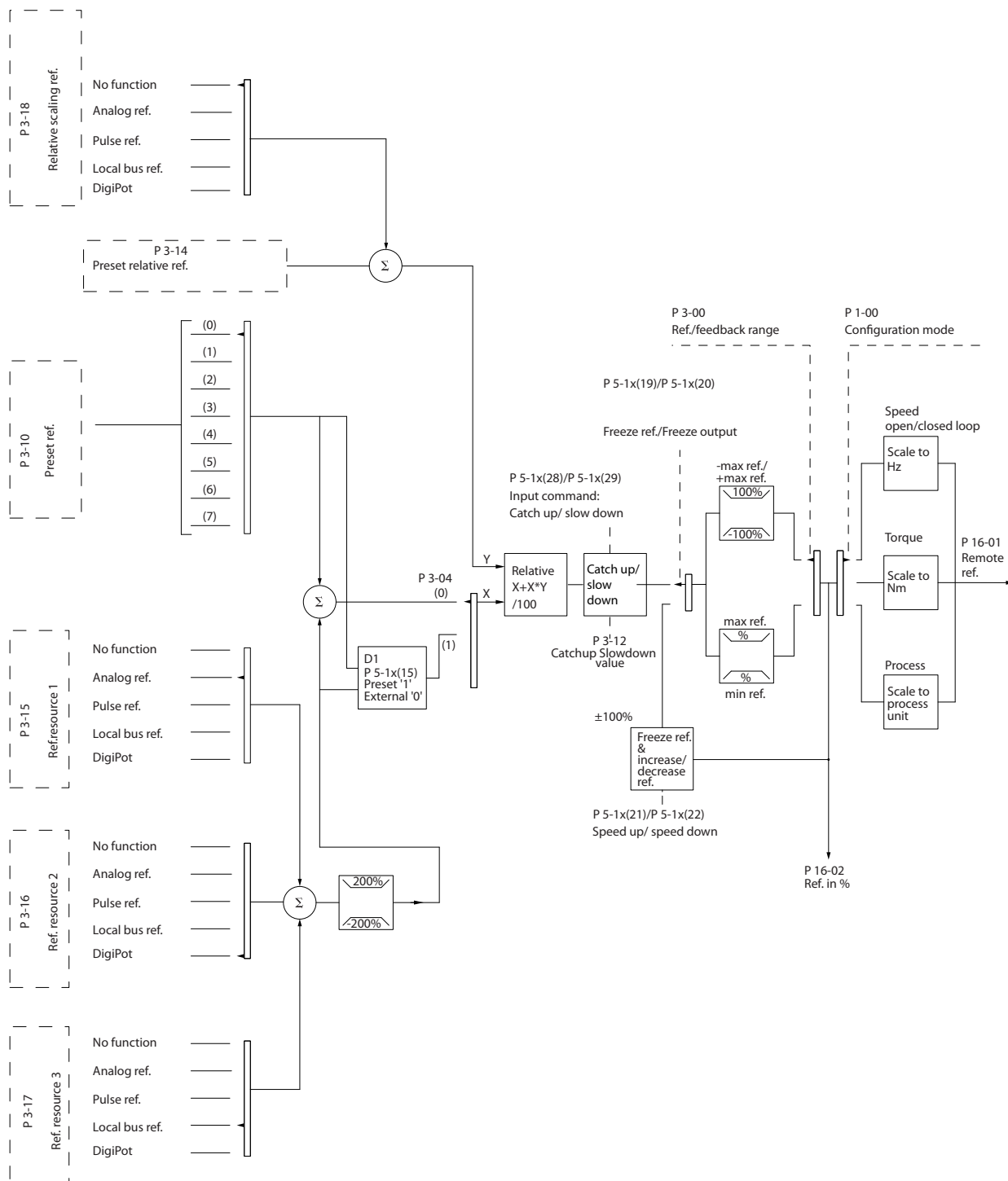
Illustration 2.16 Remote Reference
