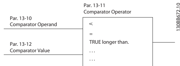
Illustration 2.38 Comparators
