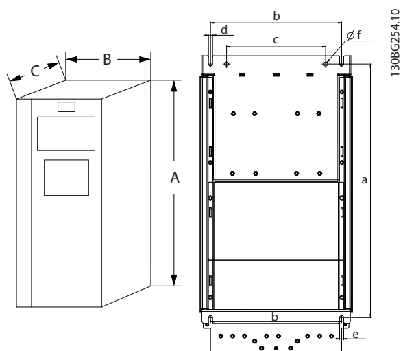
Illustration 4.12 Top and Bottom Mounting Holes J6-J7
