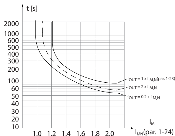
Illustration 2.40 ETR
