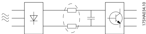
Illustration 3.53 Bobines CC
