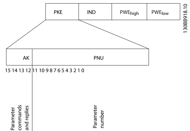
Illustration 7.9 Champ PKE
