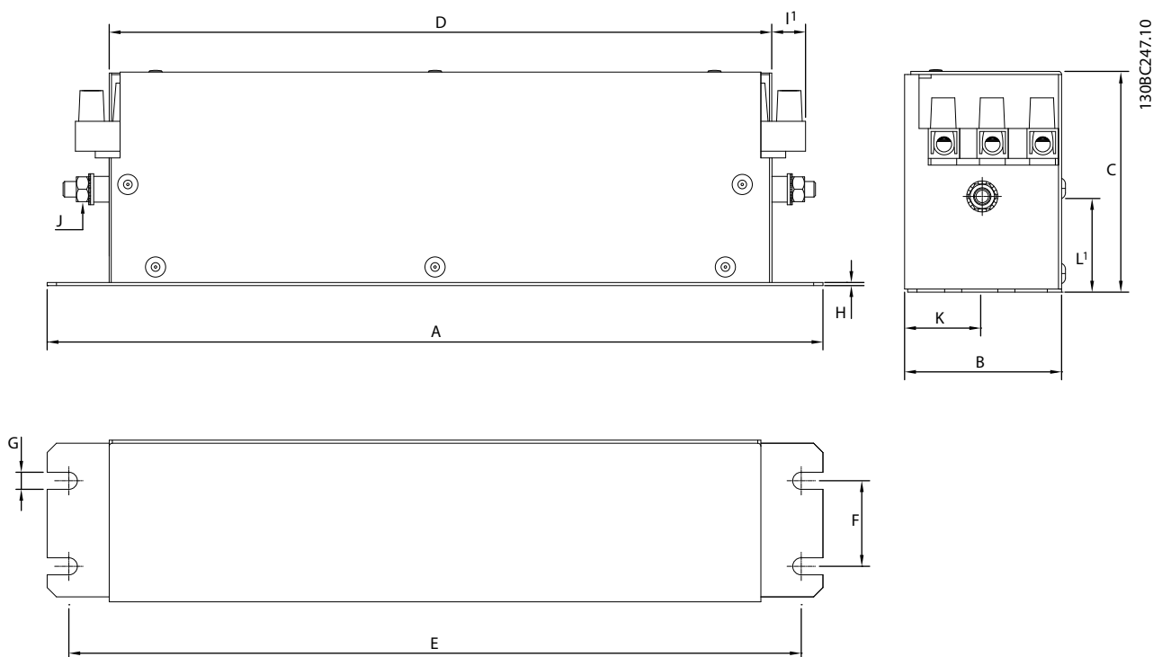
Illustration 4.9 Filtre RFI - Dimensions
