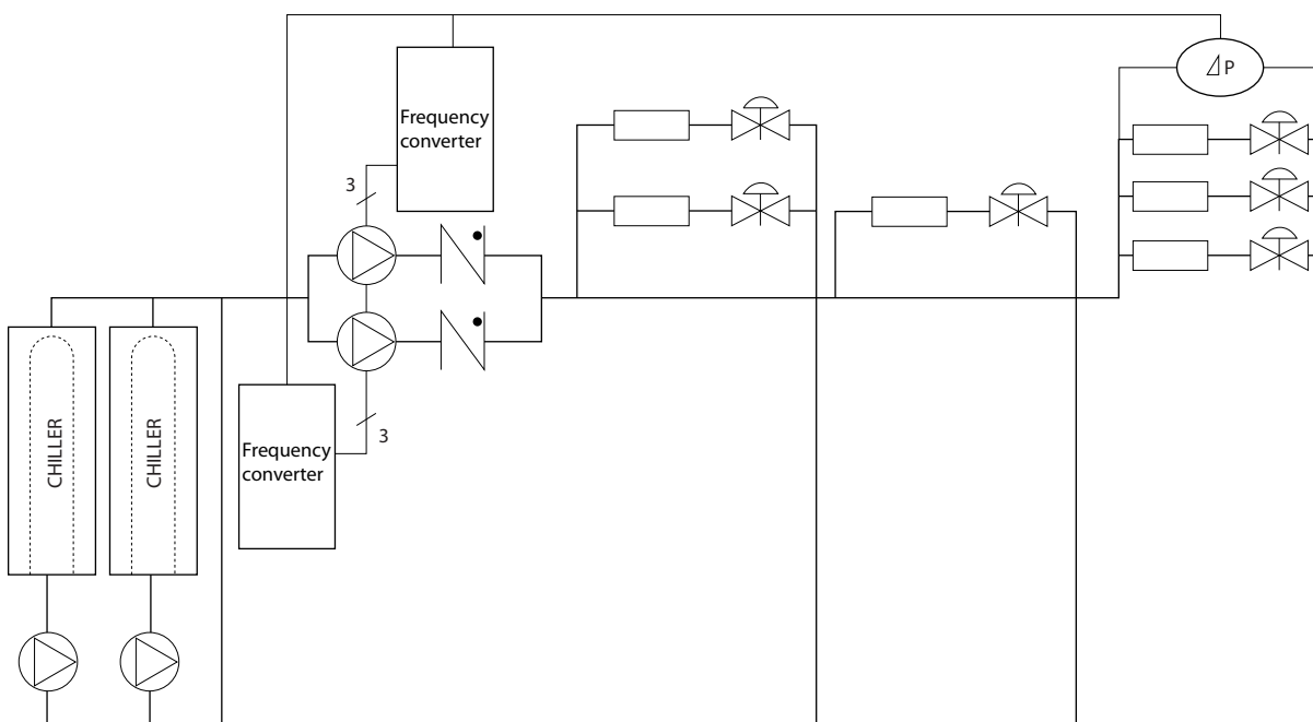
Illustration 3.16 Pompes secondaires
