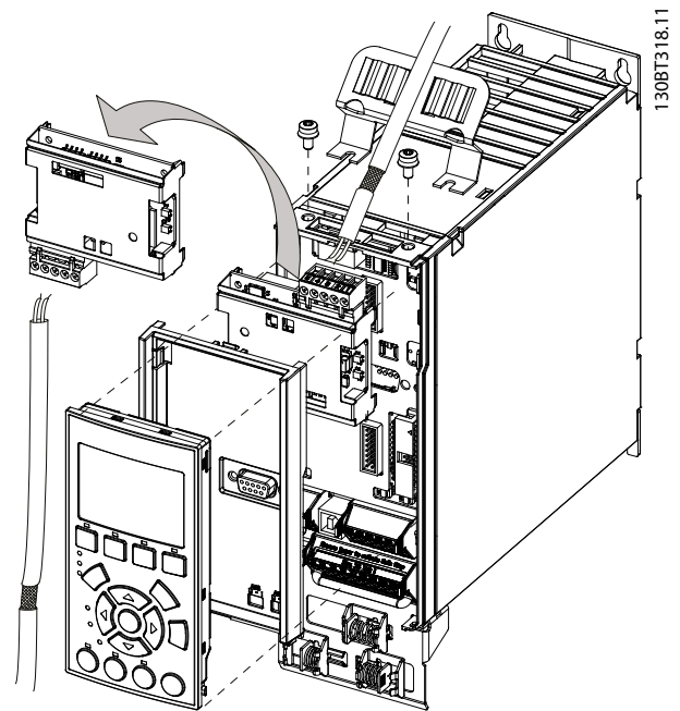
Illustration 3.2 Installing Fieldbus Option
