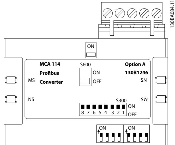
Illustration 4.1 PROFIBUS Option A
