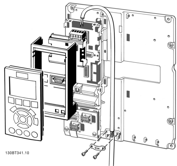
Illustration 3.3 Cable Holders
