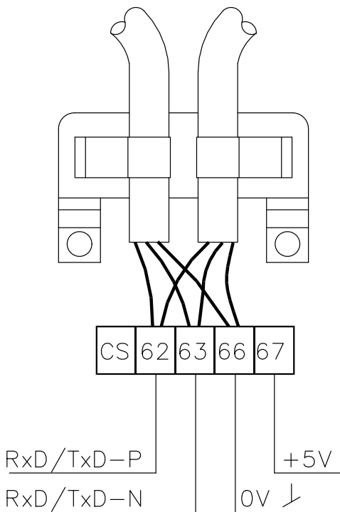
Illustration 3.1 Connecting Bus Wires to VLT PROFIBUS Converter MCA 114
