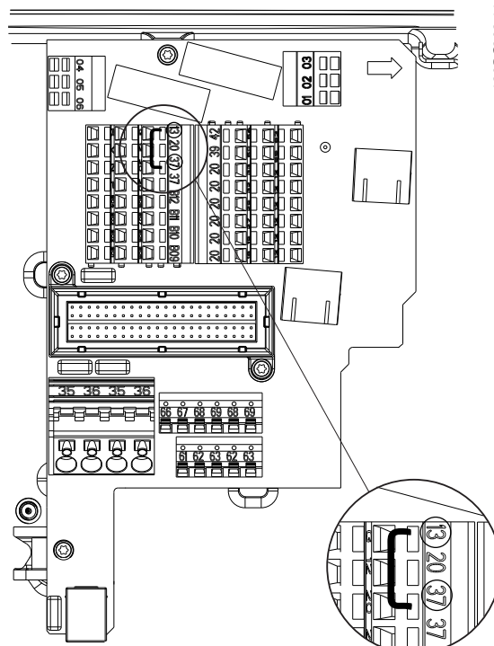
Illustration 3.2 Jumper between Terminals 13 (24 V) and 37 (FCD 302)
