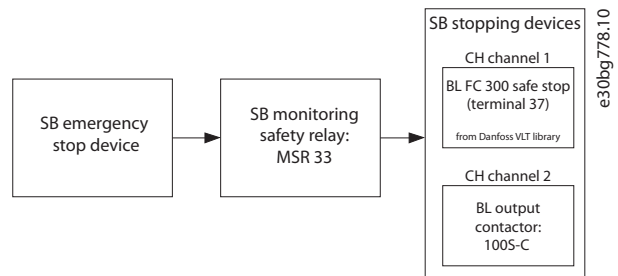
Illustration 5.6 Safety-related Block Diagram
