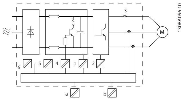
Illustration 2.14 Isolation galvanique
