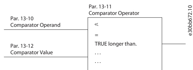
Illustration 35: Comparators
