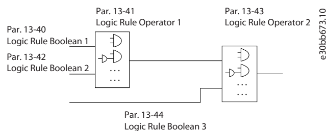
Illustration 36: Logic Rules
