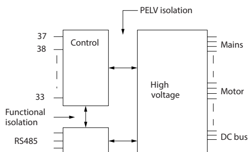
Illustration 9.1 Isolation galvanique
