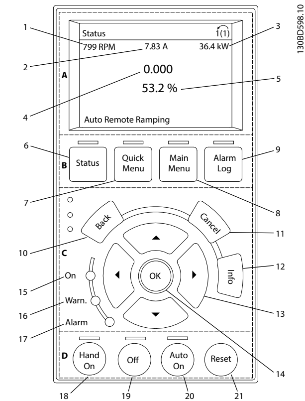
Illustration 5.1 GLCP
