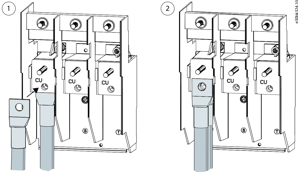
Illustration 2: Installation of 2 nd Cable
