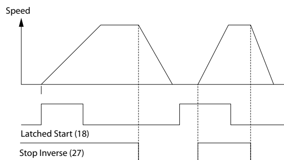
Illustration 12.2 Latched Start/Stop Inverse
