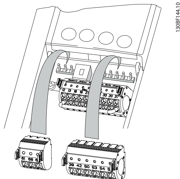
Illustration 10.6 Control Terminal Locations
