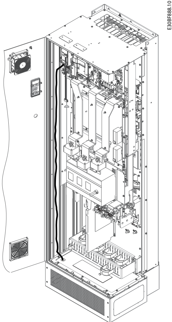
Illustration 10.5 Control card wiring path for the E1h. Same routing path for enclosures E2h and D1h–D8h.
