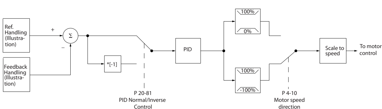
Illustration 11.7 Block Diagram of Closed-loop Controller
