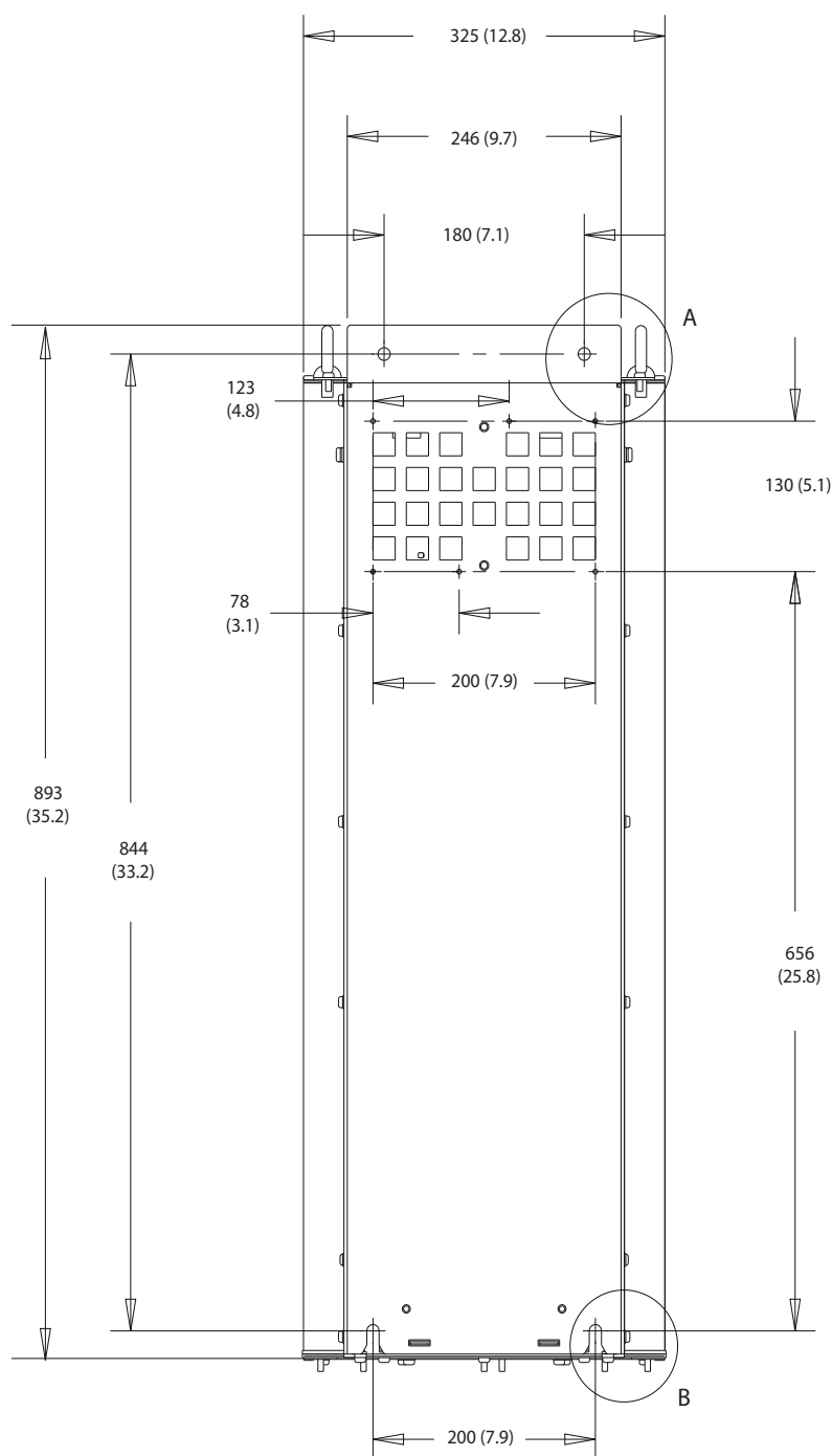
Figure 8.3 Back View of D1h
