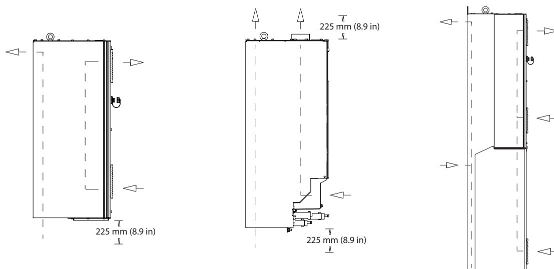
Figure 5.26 Optional Airflow Configuration Using Back-channel Cooling Kits for Enclosures D1h–D8h.
