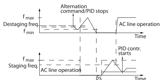
Figure 5.23 Lead Pump Alternation
