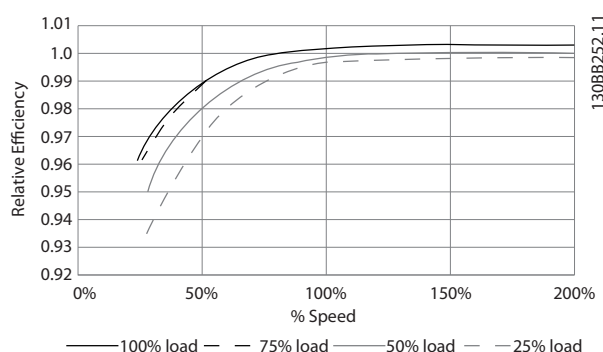
Figure 10.16 Typical Efficiency Curves
