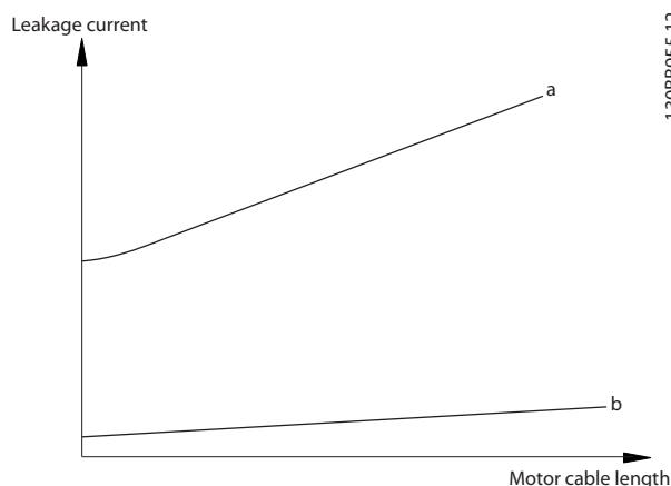
Figure 10.12 Motor cable length and power size influence the leakage current. Power size a > power size b.
