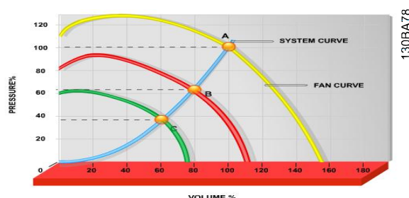
Figure 5.8 Fan Curves for Reduced Fan Volumes
