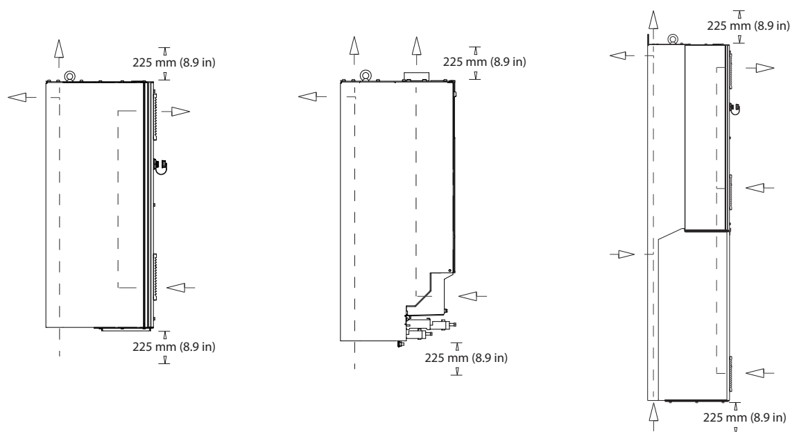
Figure 5.25 Standard Airflow Configuration for Enclosures D1h/D2h (Left), D3h/D4h (Center), and D5h–D8h (Right).
