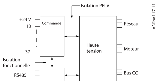
Illustration 52: Isolation PELV
