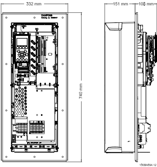
Illustration 1.9: B2 Enclosure
