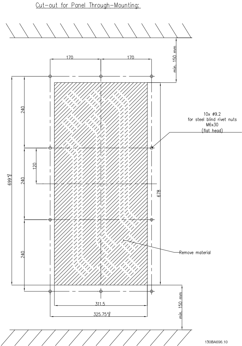
Illustration 1.4: C1 Enclosure
