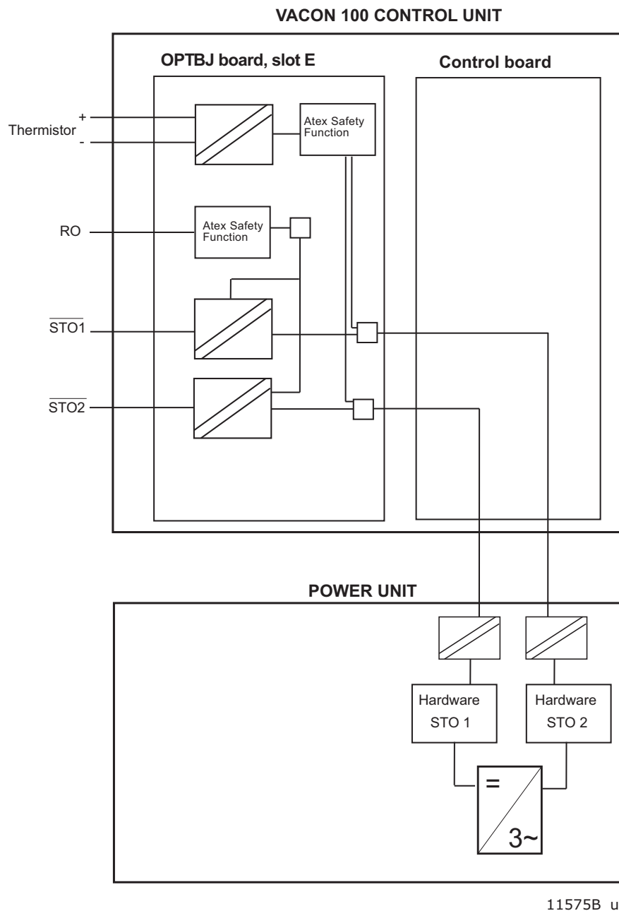
Figure 15. Thermistor function principle in VACON® 100 family AC drive with the OPTBJ board, MR4-10
