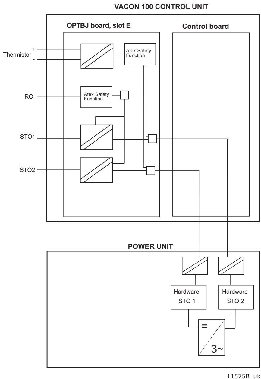
Figure 6. STO principle with OPTBJ board and VACON® 100 family control board MR4-10
