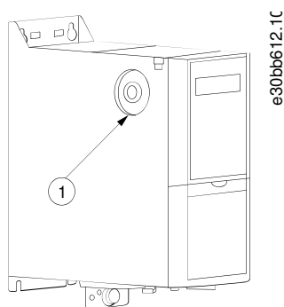
Obrázek 2: IP20, 200–240 V, 0,25–11 kW (0,33–15 hp), IP20, 0,37–22 kW (0,5–30 hp), 380–480 V
