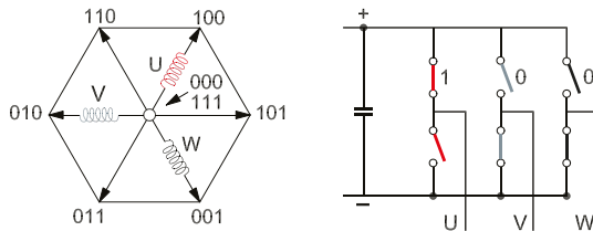
Fig. 3.16 Inverter switch states
