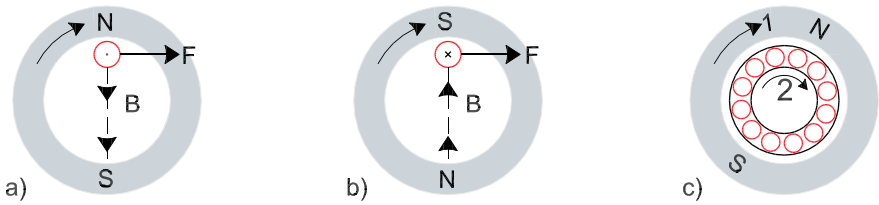
Fig. 2.12 Induction in the rotor rods
