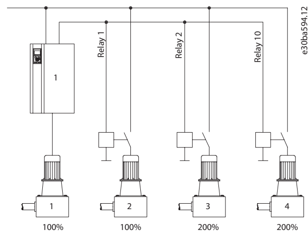
Illustration 5.8 Application Overview
