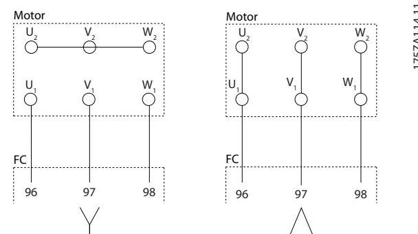
Illustration 10.5 Motor Cable Connection
