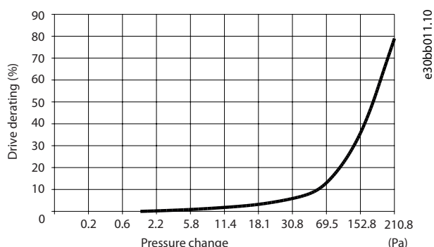
Illustration 9.6 Derating vs. Pressure Change for E1-E2 Enclosures, 380–480 V Models: P355–P450 and 525–690 V Models: P560–P630. Airflow: 850 cfm (1445 m 3 /h)
