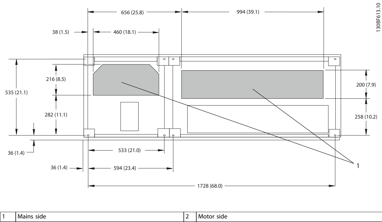
Illustration 8.27 Gland Plate Dimensions for F2
