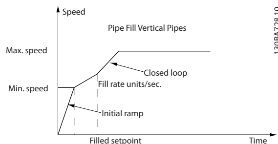
Illustration 12.6 Performance Curve for Pipe Fill Mode
