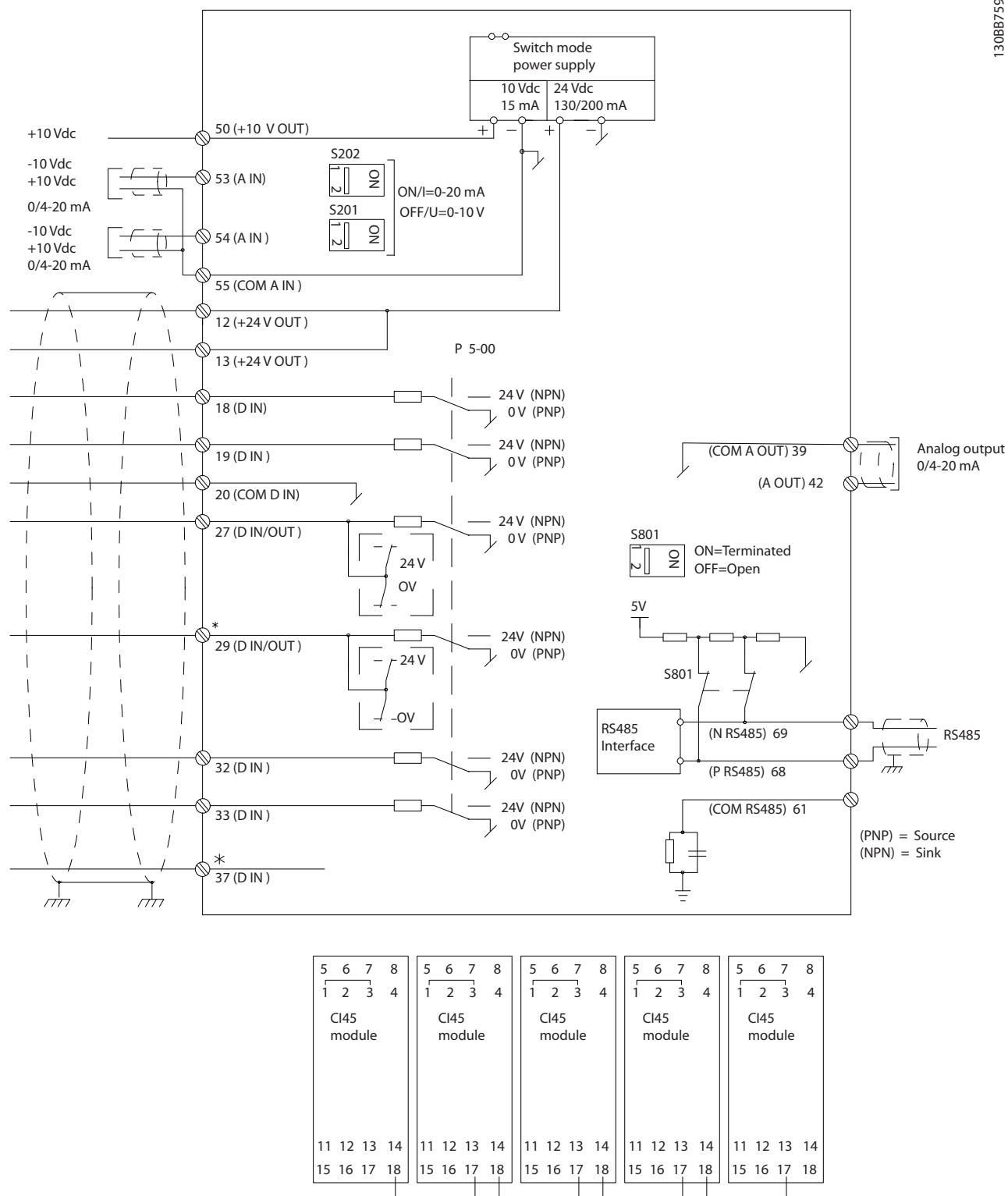
Illustration 10.17 12-pulse Control Terminals
