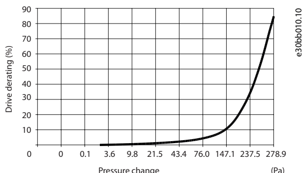
Illustration 9.5 Derating vs. Pressure Change for E1-E2 Enclosures, 380–480 V Models: P315 and 525–690 V Models: P450–P500. Airflow: 650 cfm (1105 m 3 /h)
