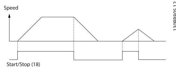
Illustration 12.1 Start/Stop with Safe Torque Off
