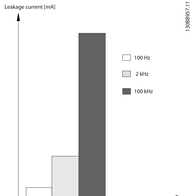
Figure 10.24 Influence of the RCD Cut-off Frequency on Leakage Current
