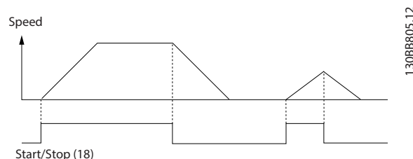
Figure 12.1 Start/Stop with Safe Torque Off
