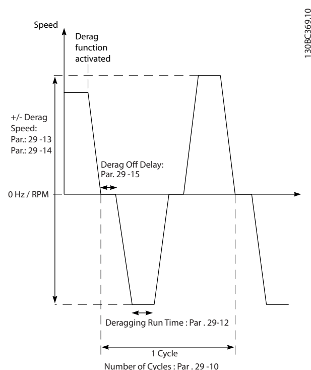
Figure 5.12 Derag Function
