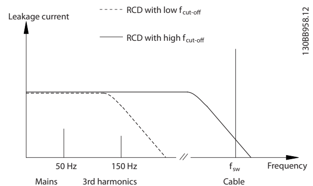
Figure 10.23 Main Contributions to Leakage Current
