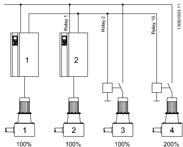
Figure 5.7 Application Overview
