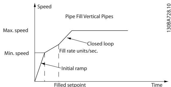
Figure 12.6 Performance Curve for Pipe Fill Mode
