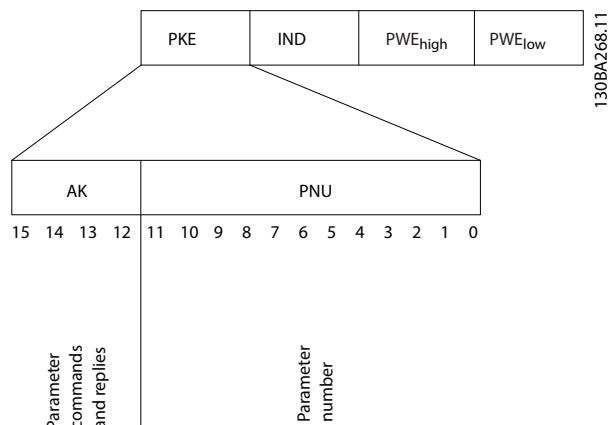
Figure 14.10 PKE Field
