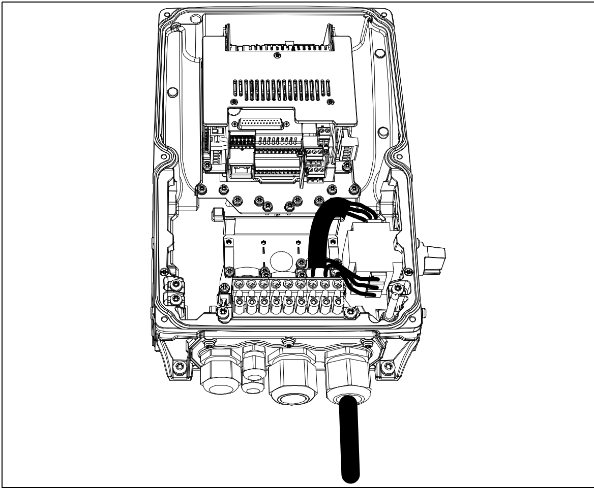
Figure 7. Mains switch, cable entry and cables connected.
