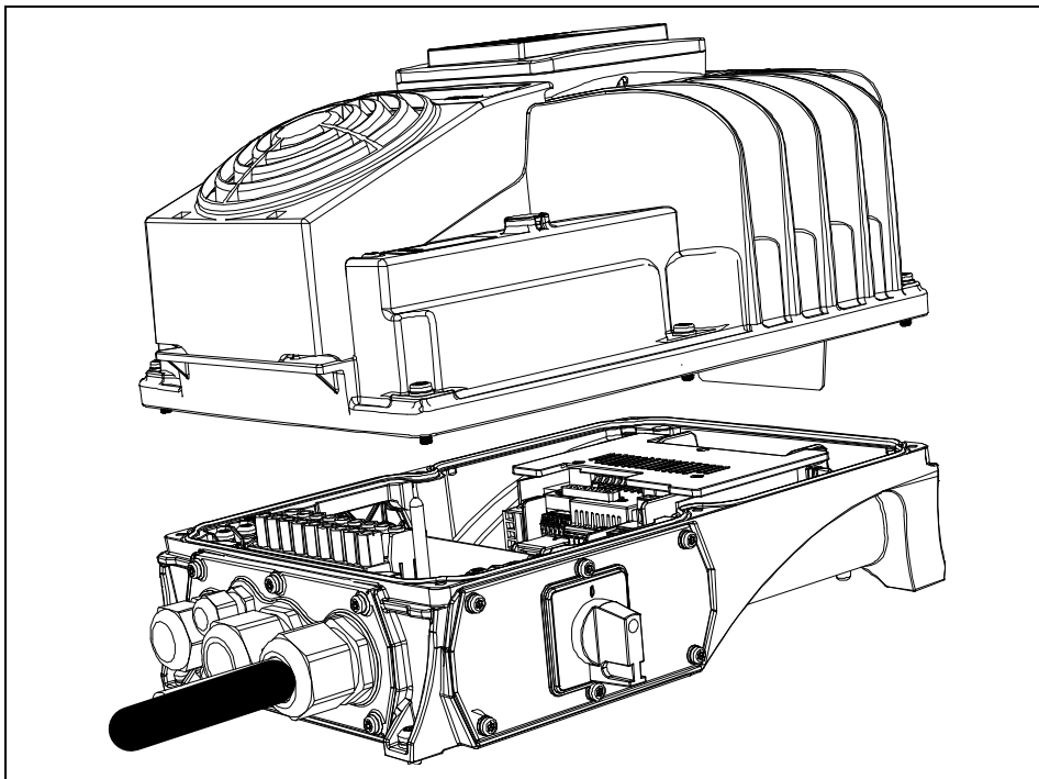
Figure 8. Mount the powerhead on the terminal box.
