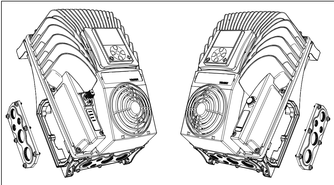
Figure 3. The mains switch can be mounted on either side of the drive. Disconnect the cable entry plate in which mains switch has to be mounted: example for MM5.
