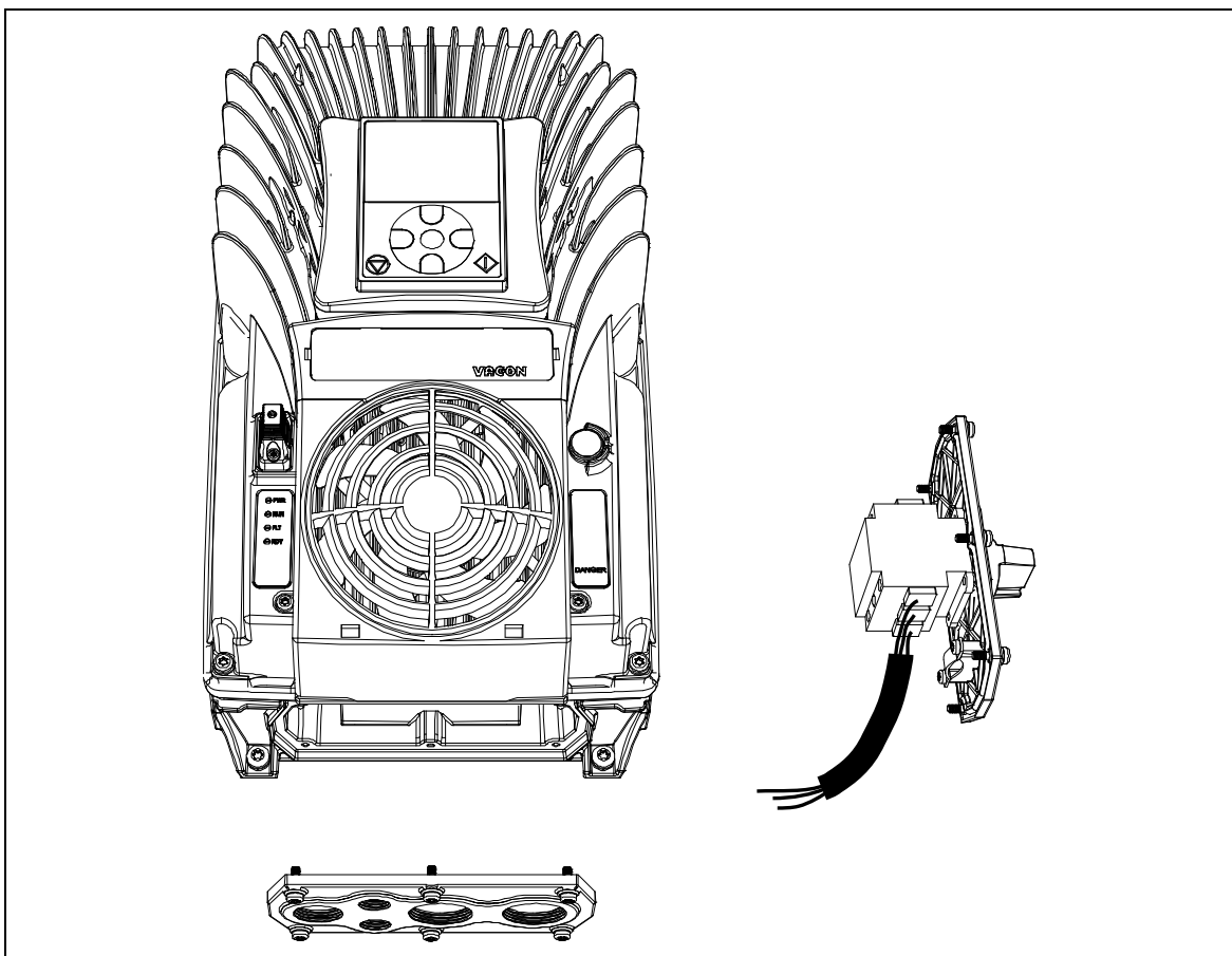
Figure 4. Cable entry plate from the bottom side of the drive from which the cables enter.
