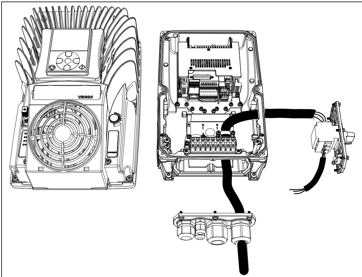
Figure 6. Connection of the supply cable to the Mains switch (right-hand-side example).
