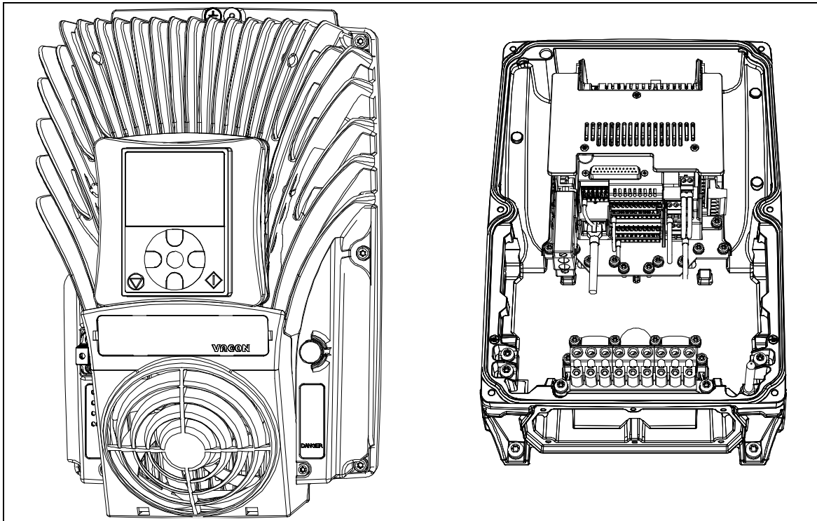
Figure 5. Powerhead separated from the terminal box.
