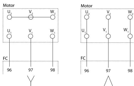
Illustration 10.3 Motor Cable Connection
