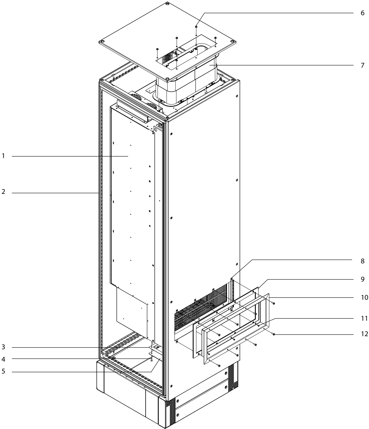
Illustration 2: Overview of In-back/Out-top Cooling Kit
