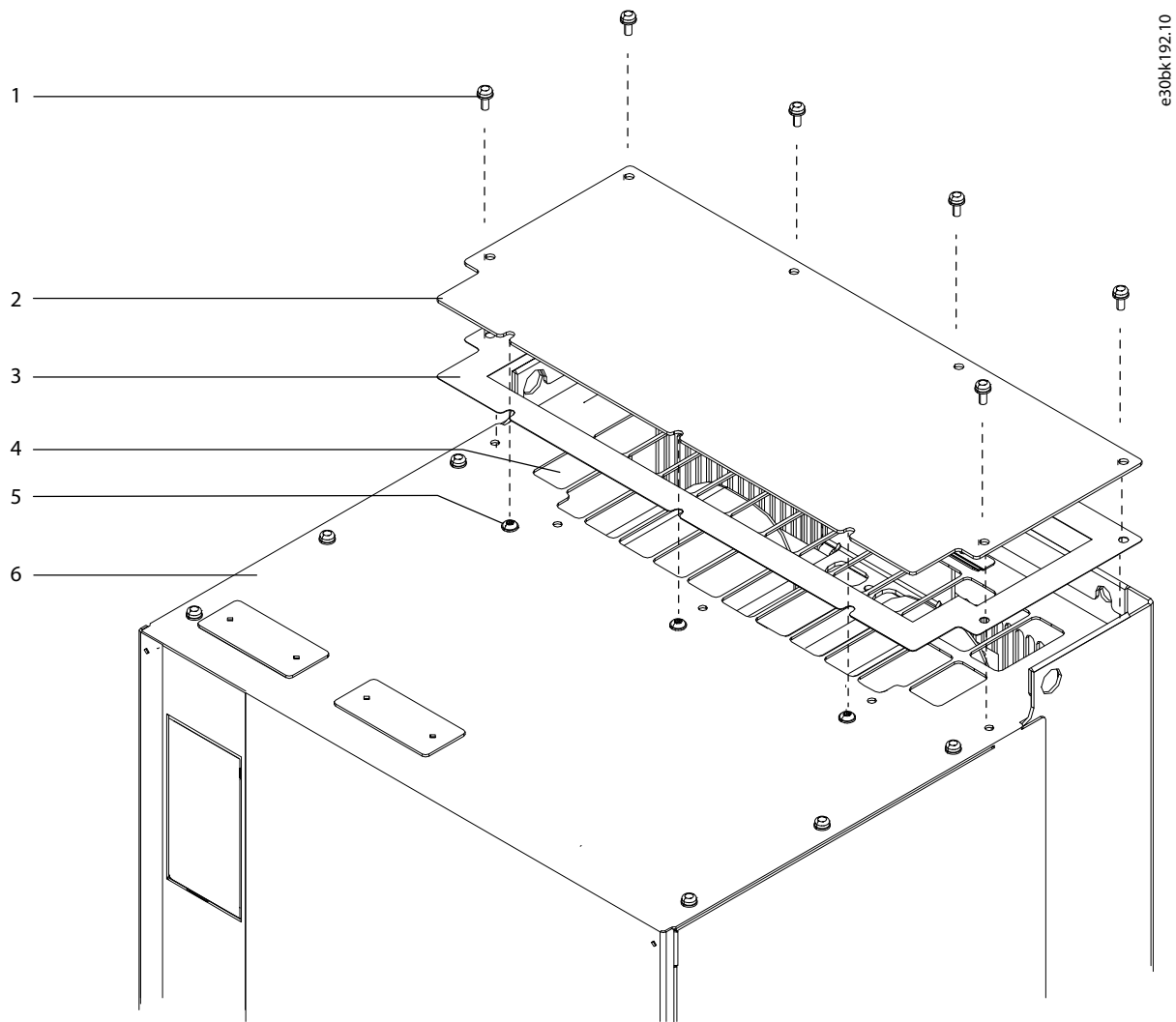
Illustration 8: Installation of Top Cover
