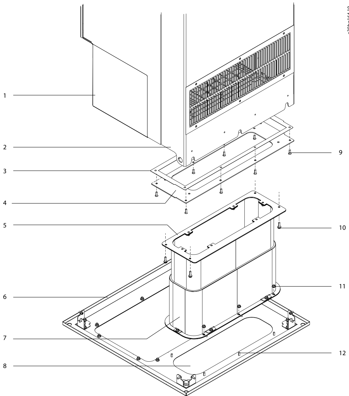
Illustration 10: Installation of the Duct Support Bracket
