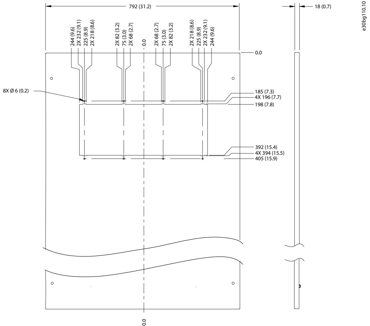
Illustration 7: Vent Template for Backplate in 800 mm (32 in) Cabinet
