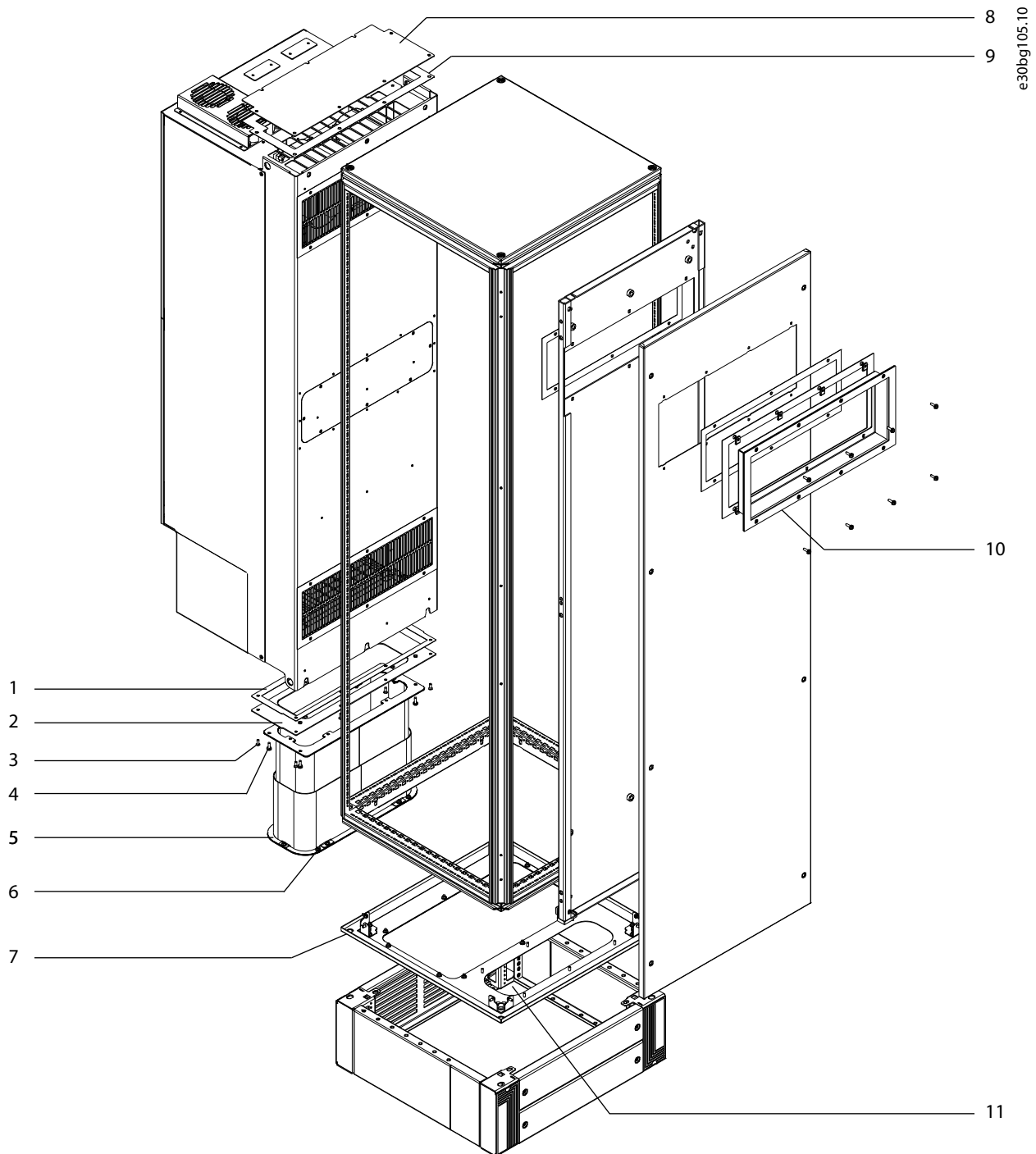
Illustration 2: Overview of In-bottom/Out-back Cooling Kit
