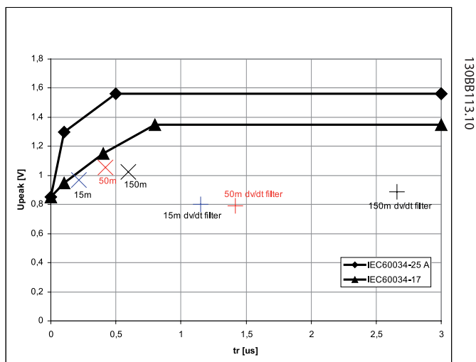
Illustration 3.3: Measured du/dt values (rise time and peak voltages) with and without du/dt filter using 15 m, 50 m and 150 m cable lengths on a 400 V, 37 kW induction motor.
