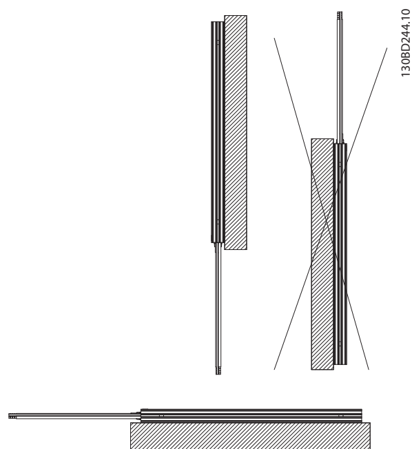
Illustration 9.38 Mechanical Mounting
