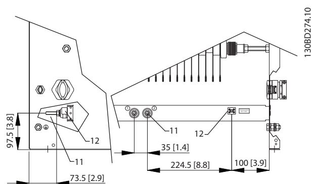
Illustration 9.67 Connections
