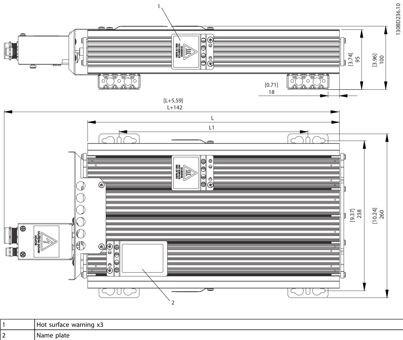
Illustration 9.1 IP21, Side View and Top View
