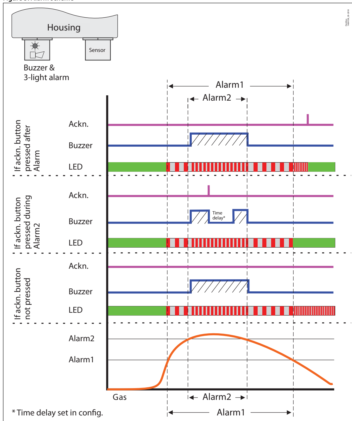
Figure 5: Alarm scheme
