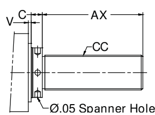
Type #M Extended Int. Male UN Thread
