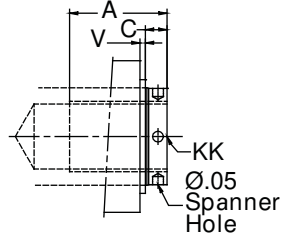
Type #9 Intermediate Male UN Thread
