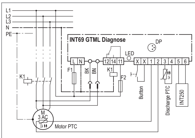
Wiring diagram
