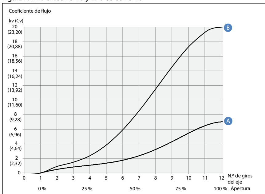
Figura 7: REG-SA SS 25-40 y REG-SB SS 25-40
