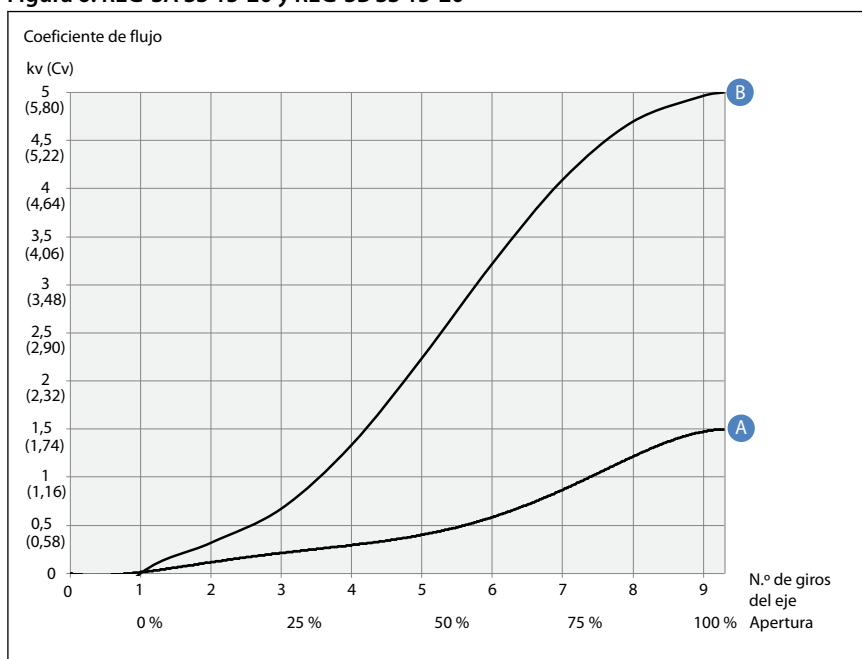
Figura 7: REG-SA SS 25-40 y REG-SB SS 25-40
