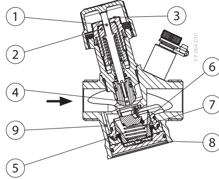
AB-QM DN 15-32
