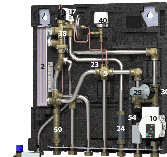
MSS 1, 2, 3 with circulation
