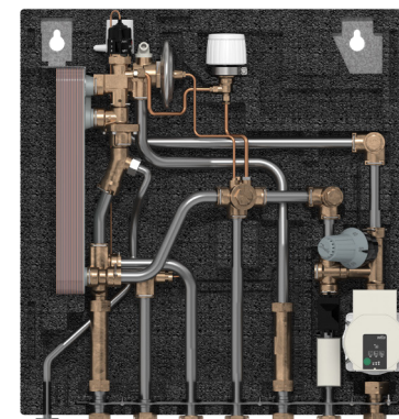
EvoFlat MSS, with circulation
