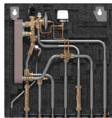
EvoFlat FSS, with circulation
