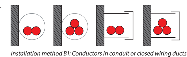
Installation method B1: Conductors in conduit or closed wiring ducts
