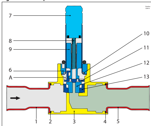
Figure 2: Servo operated
