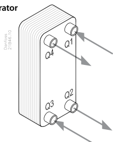
Dual Circuit Evaporator
