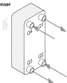
Dual Circuit Condenser
