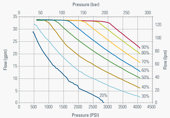
Flow vs Pressure - 74cc
