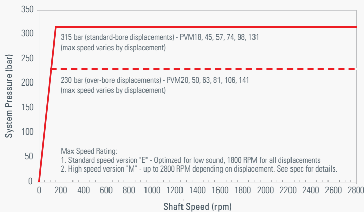
PVM System Pressure vs. Shaft Speed
