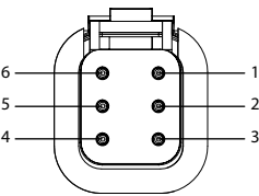
Pin connector
