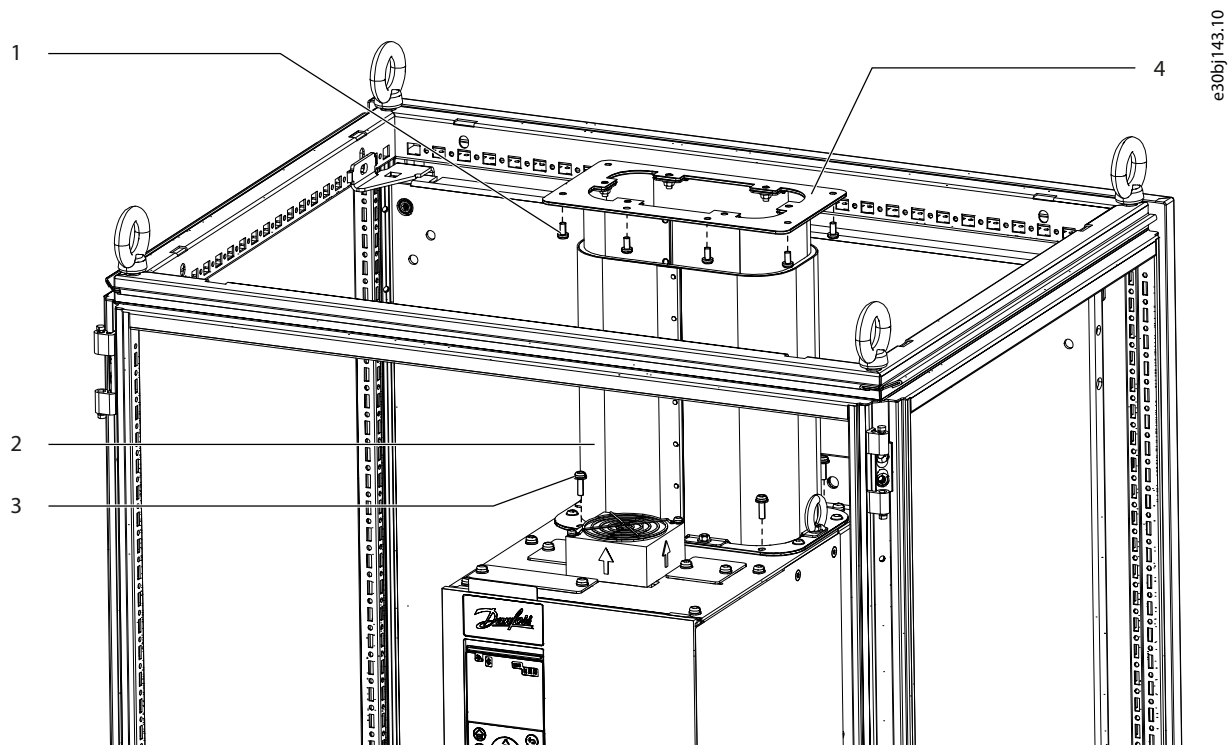
Illustration 13: Installation of the Top Duct
