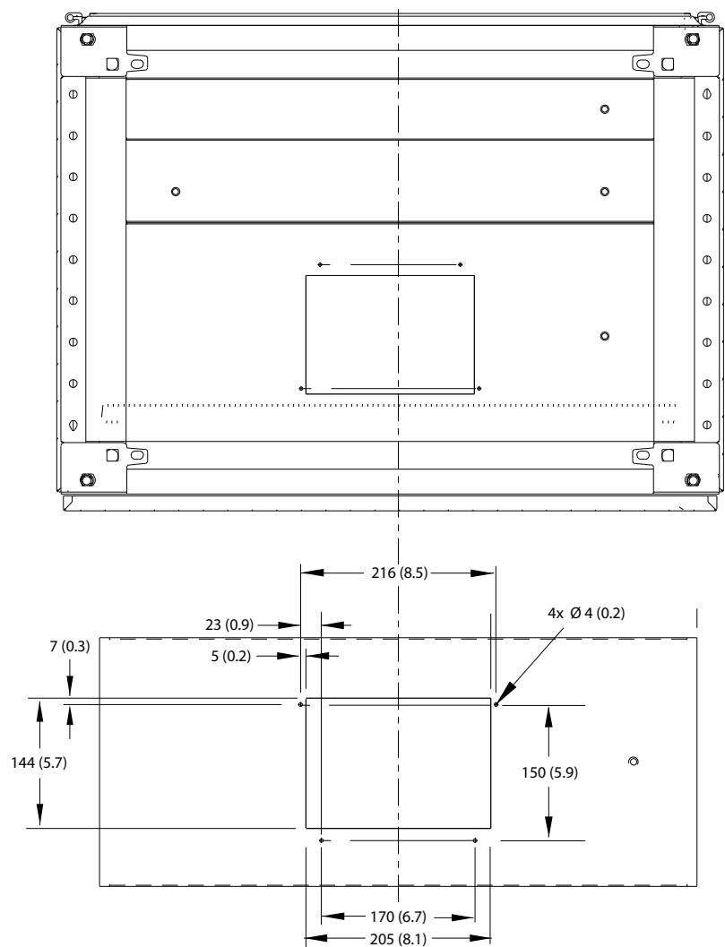
Illustration 5: FA09 Base Plate Template
