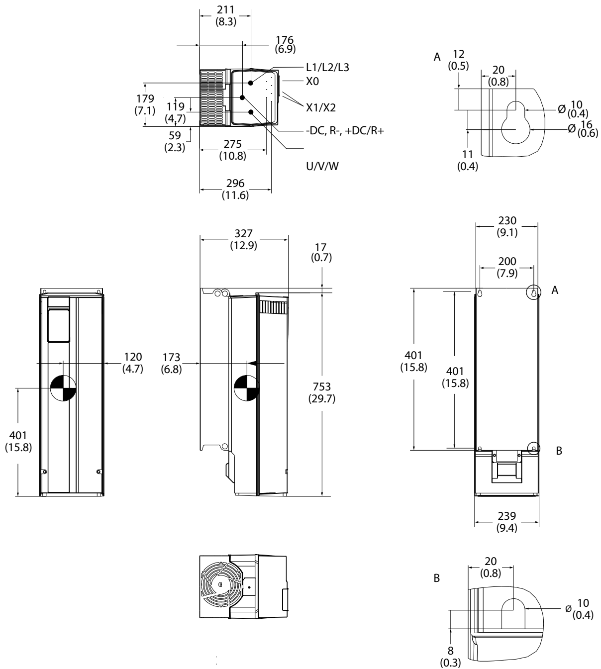
Illustration 21: Dimensions de FK07
