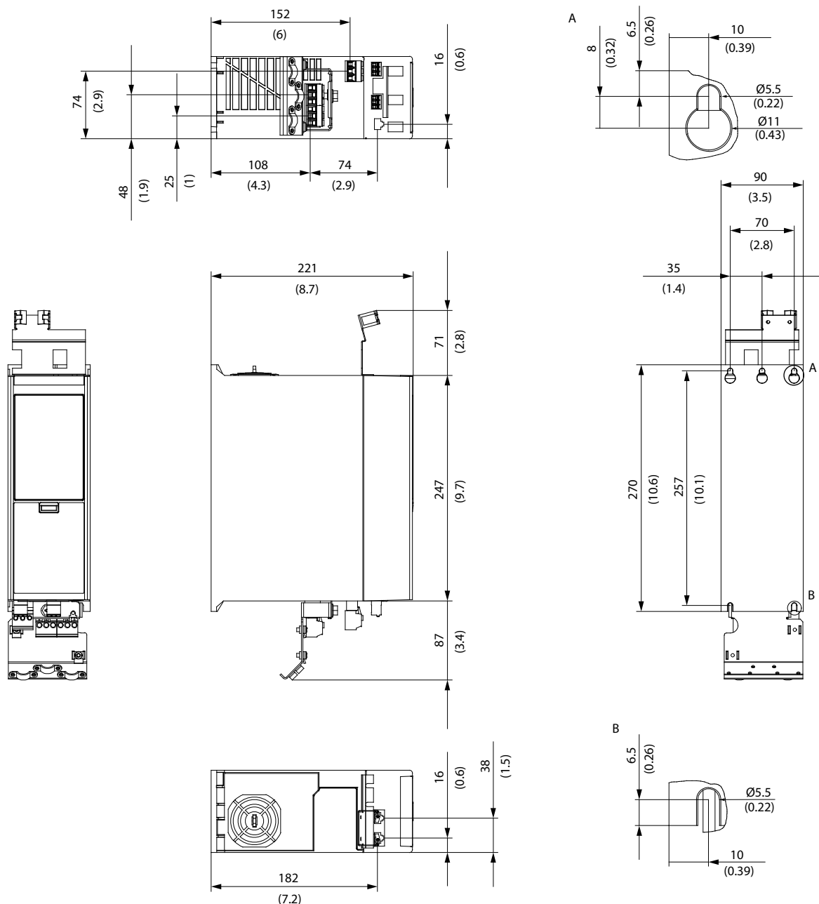
Illustration 10: Dimensions de FA02a
