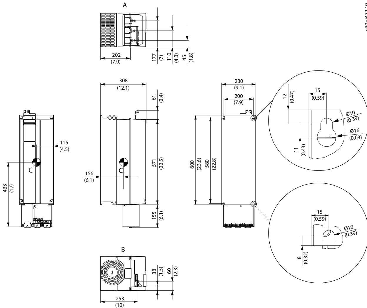
Illustration 19: Dimensions de FA07
