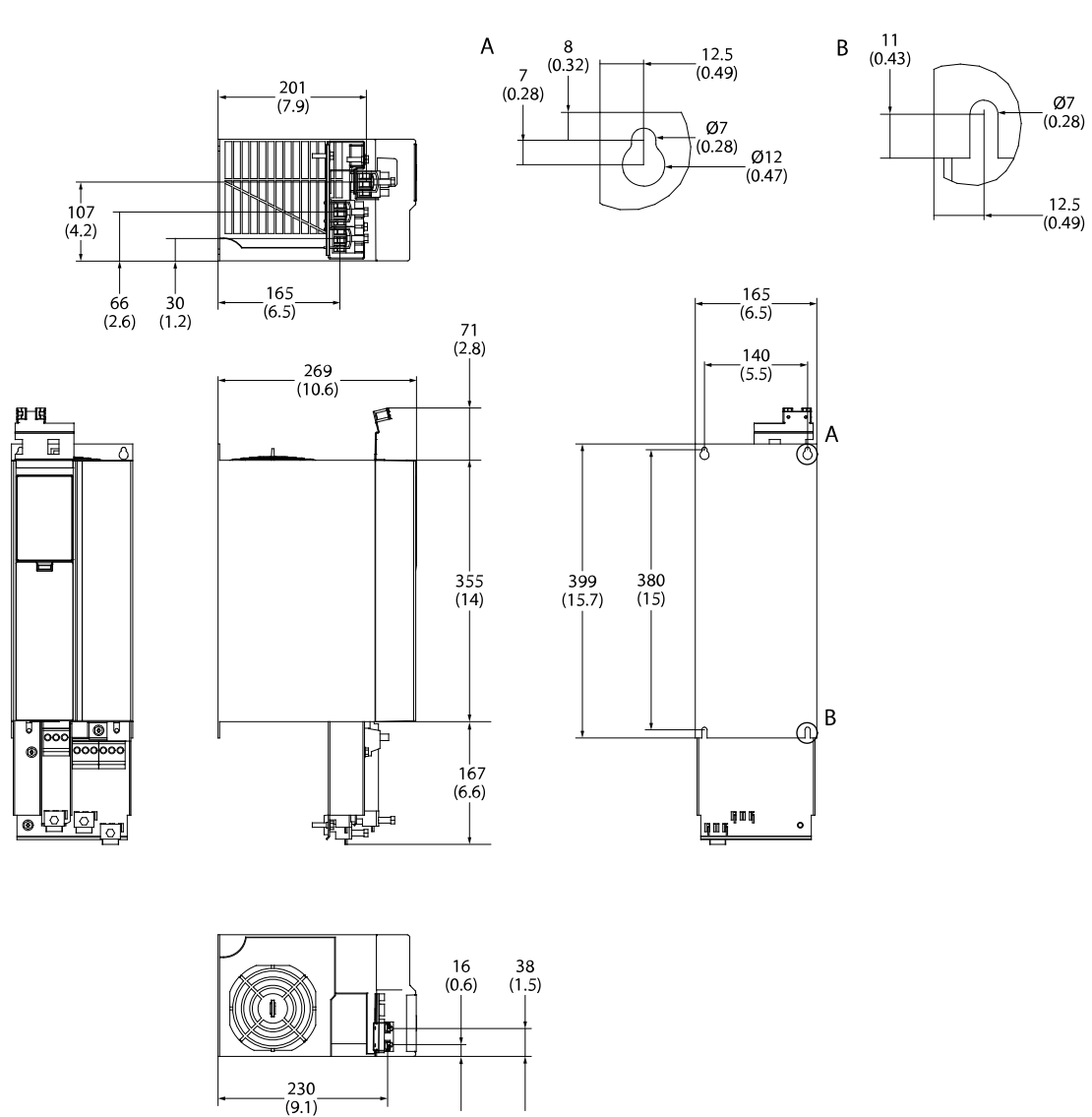
Illustration 16: Dimensions de FA05a
