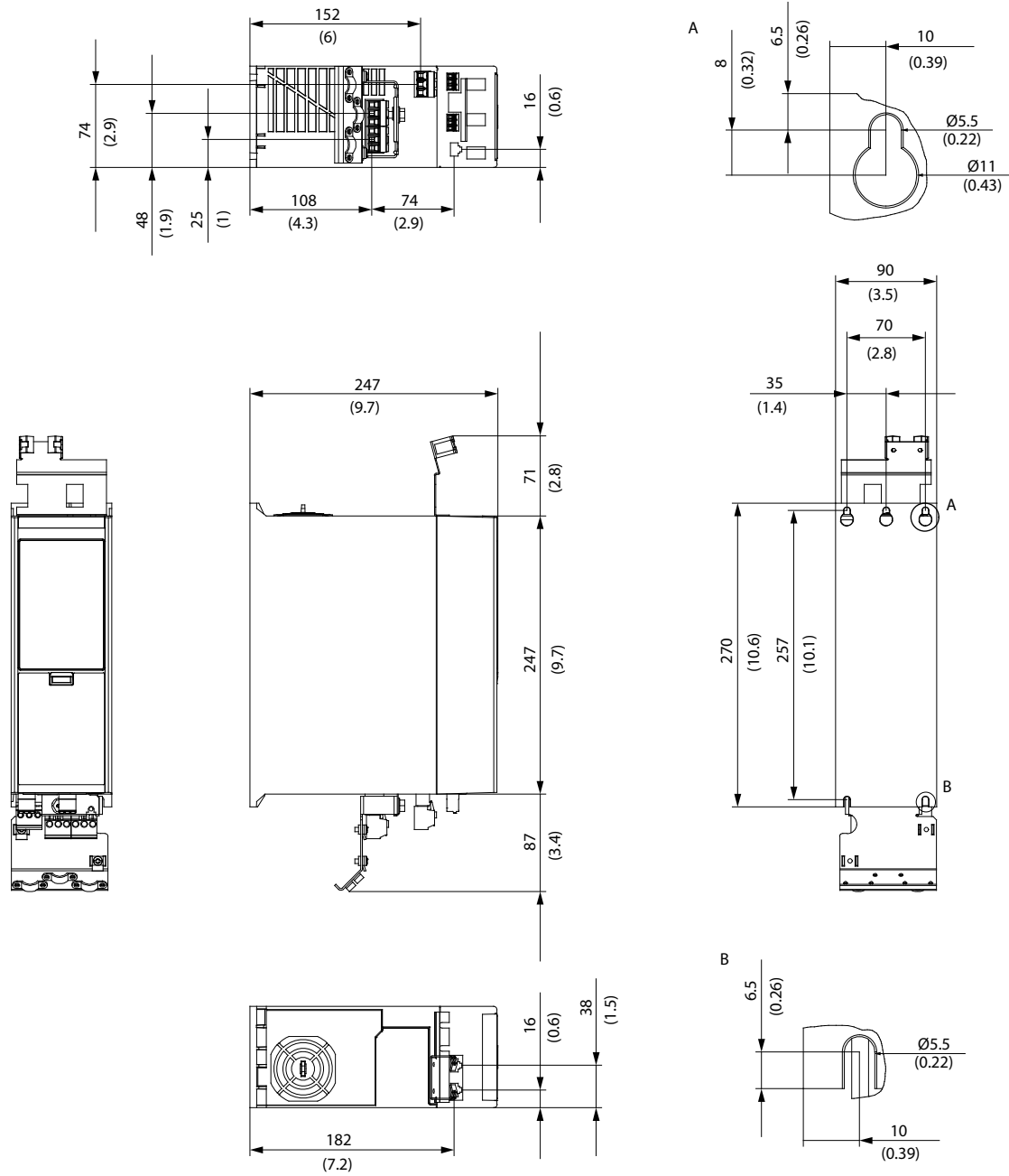
Illustration 11: Dimensions de FA02b
