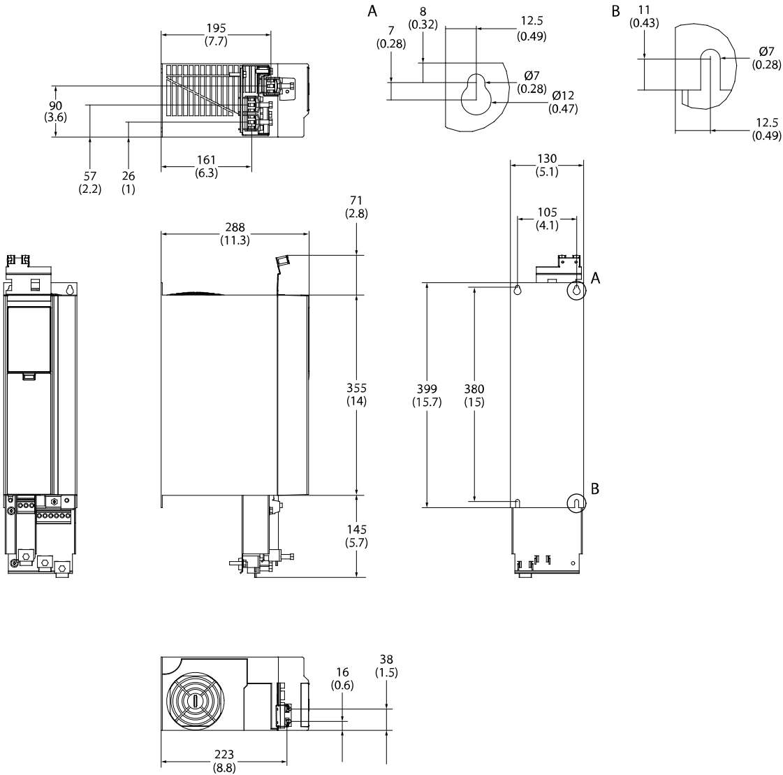
Illustration 15: Dimensions de FA04b
