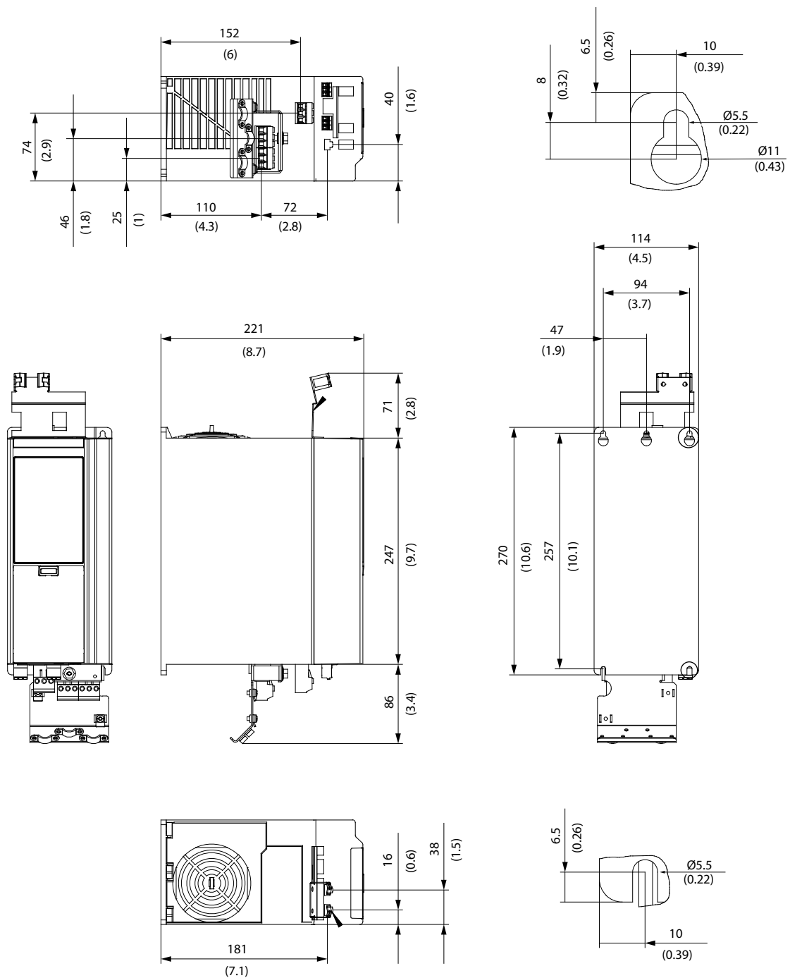
Illustration 12: Dimensions de FA03a
