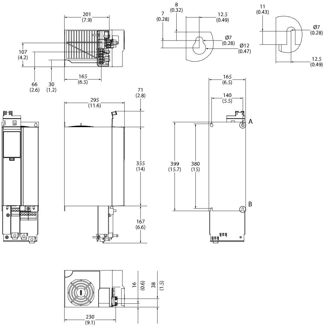
Illustration 17: Dimensions de FA05b
