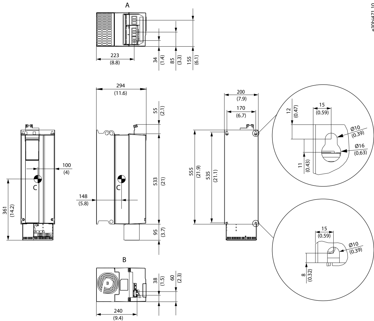
Illustration 18: Dimensions de FA06
