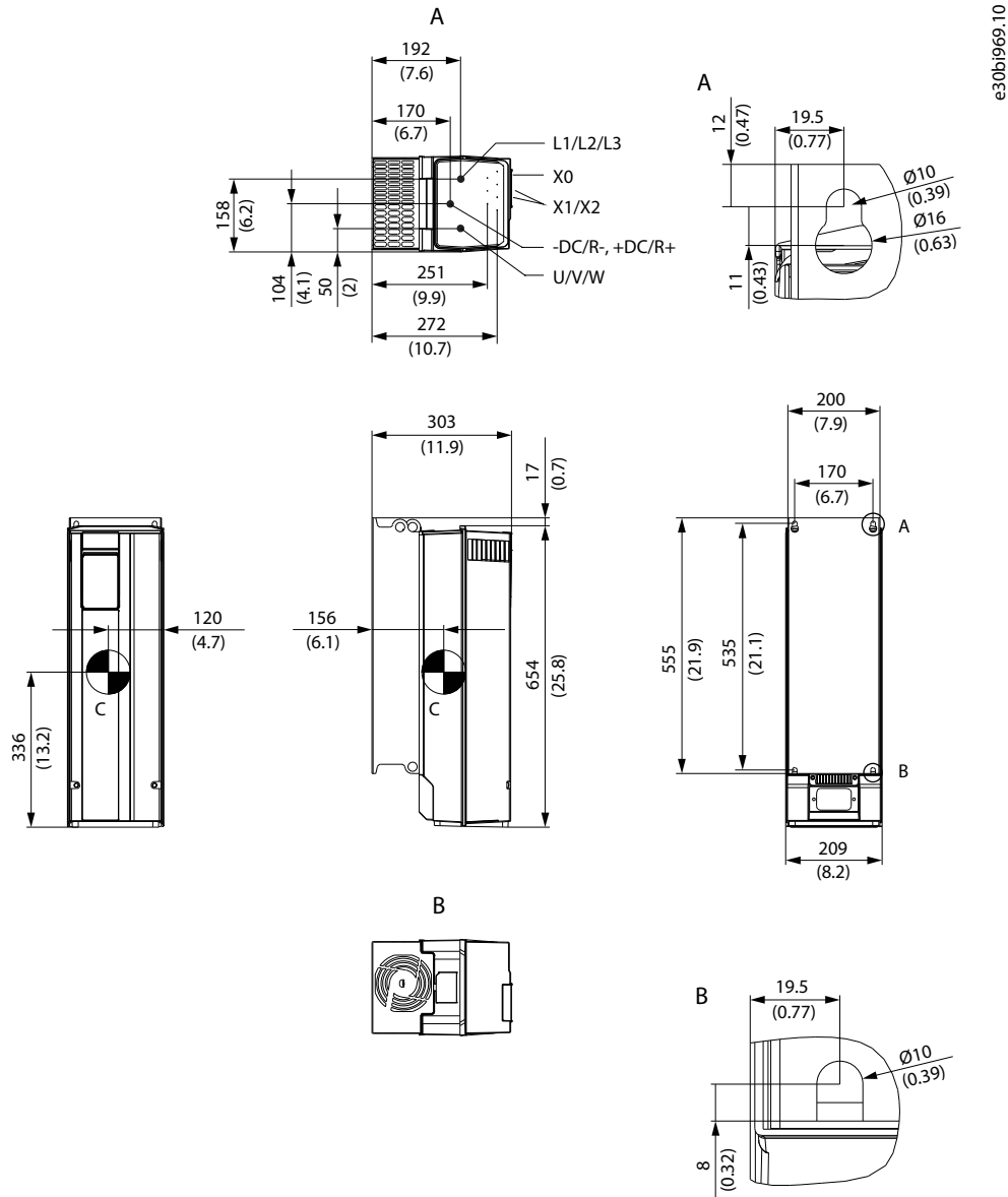
Illustration 20: Dimensions de FK06
