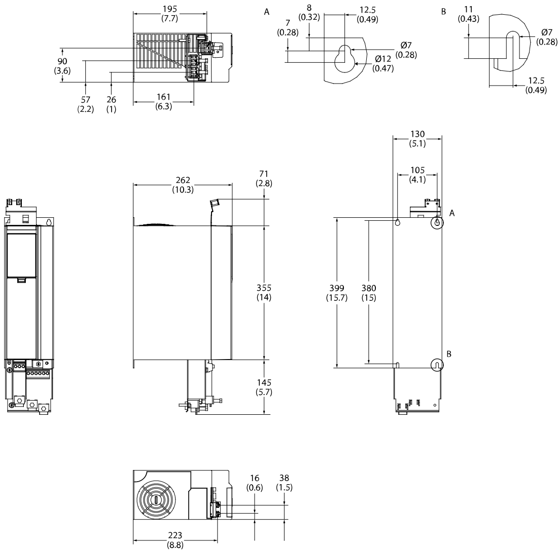
Illustration 14: Dimensions de FA04a
