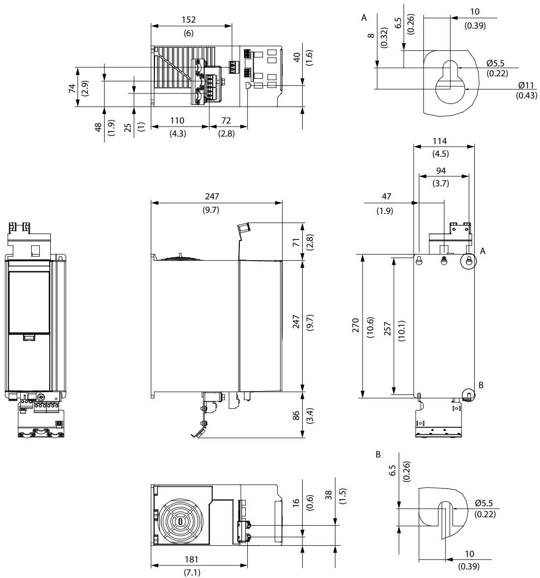
Illustration 13: Dimensions de FA03b
