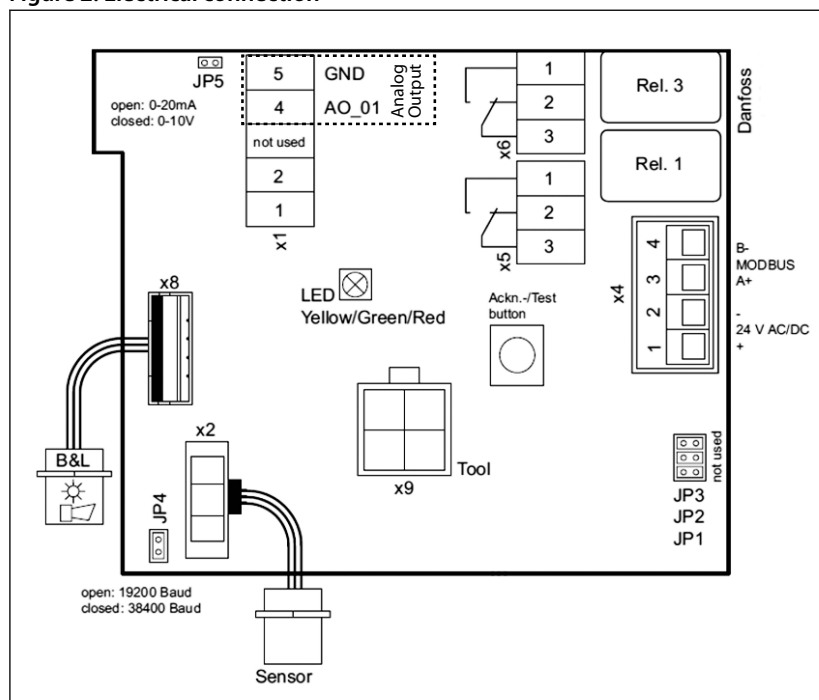
Figure 2: Electrical connection
