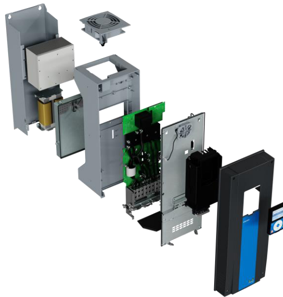
Figure 1: The exploded illustration of the drive with its main components.
