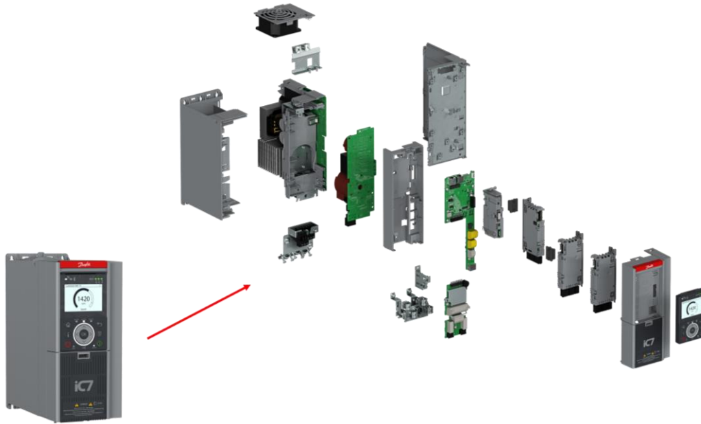
Figure 1: The exploded illustration of the drive with its main components.
