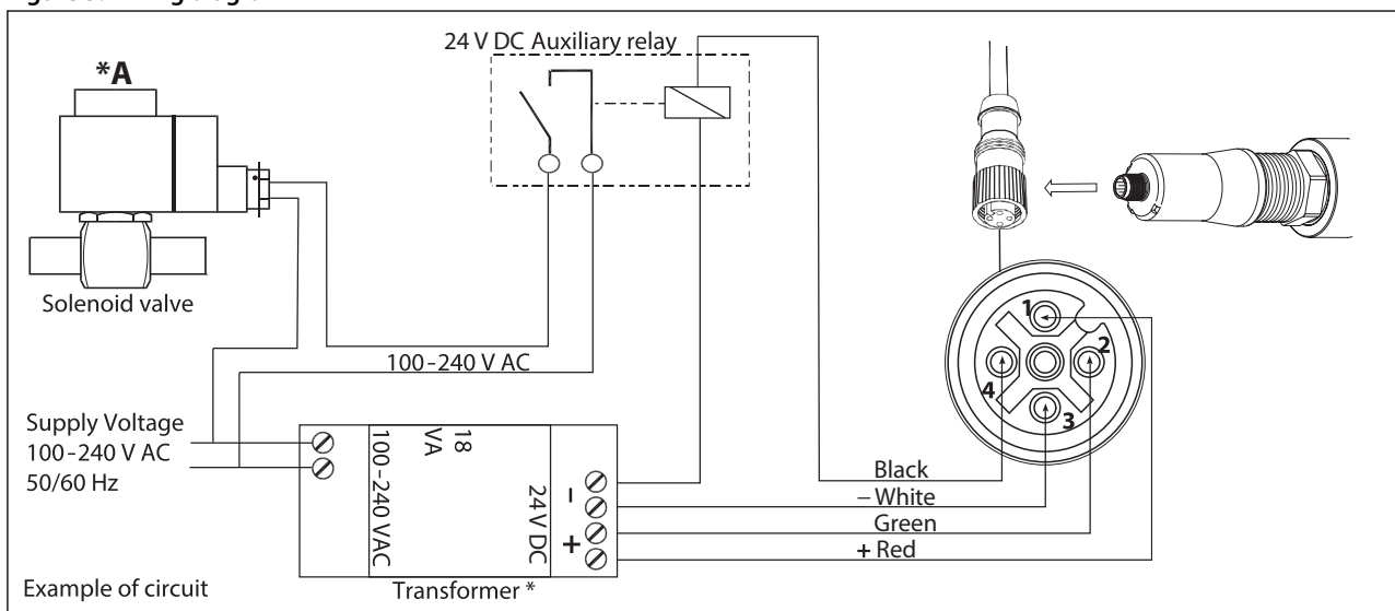
Figure 5: Wiring diagram
