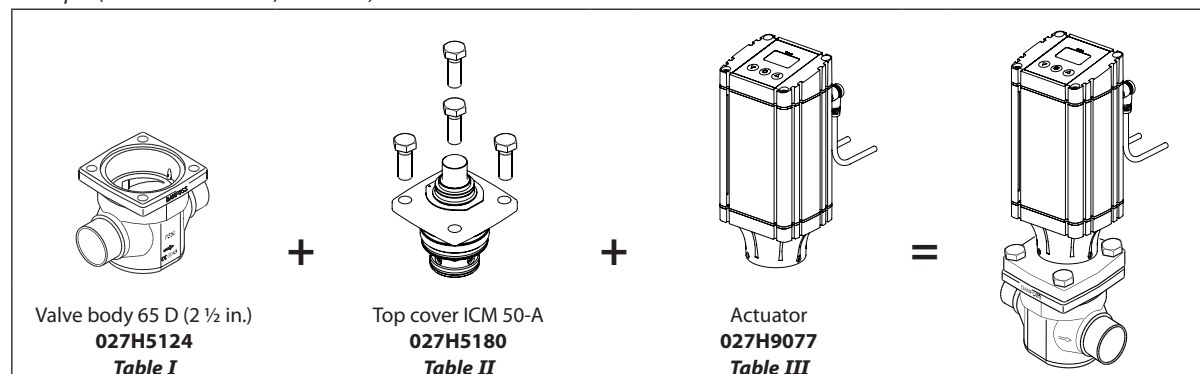
ICV 50 valve body w/different connections
