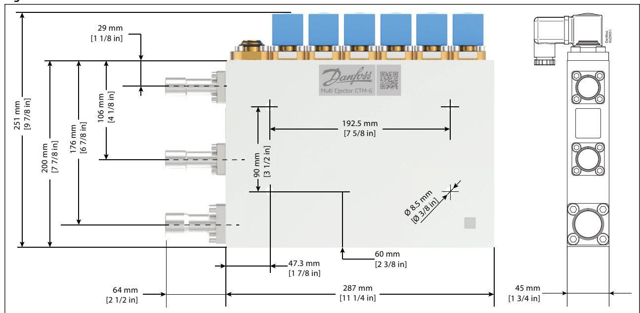
Figure 3: Dimensions
