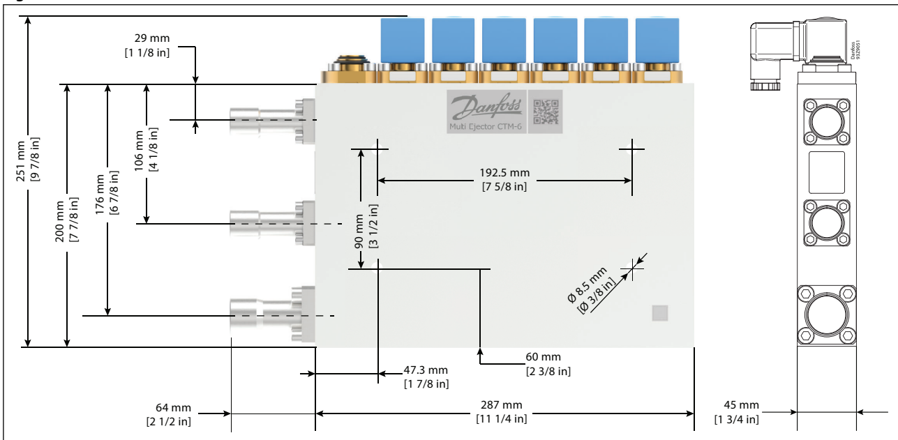
Figure 3: Dimensions
