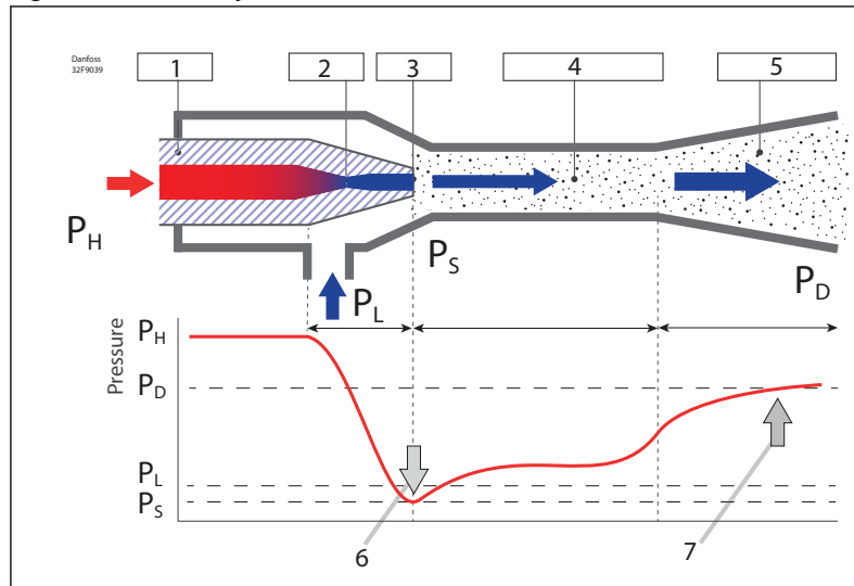
Figure 1: The Multi Ejector function
