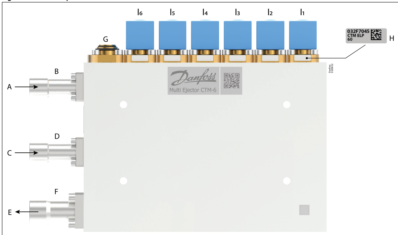
Figure 4: Connector positions
