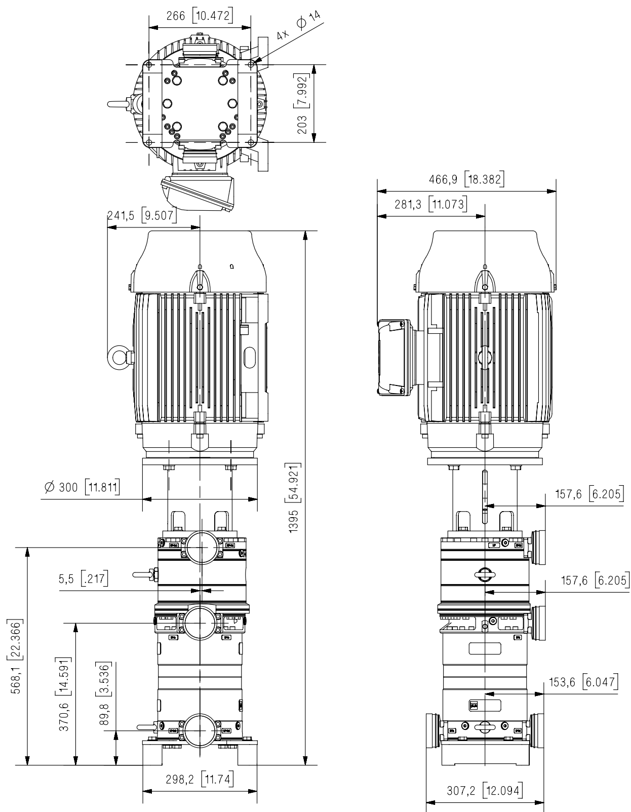
iSave 40 - vertical, 20 HP, 6 pole, NEMA motor
