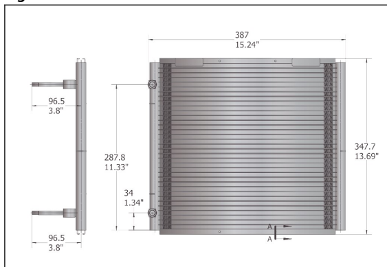
Figure 1: Dimensions
