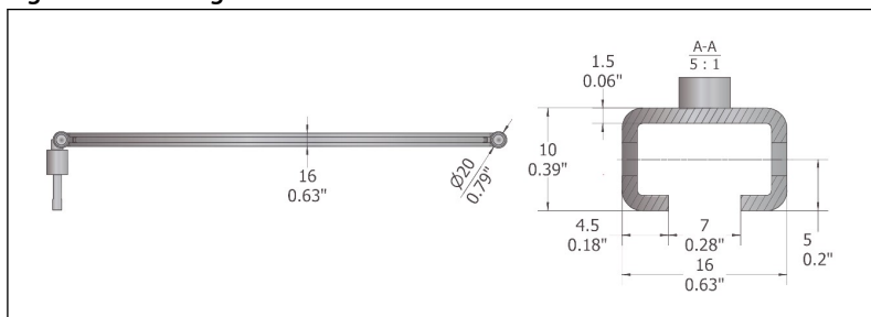
Figure 2: Mounting
