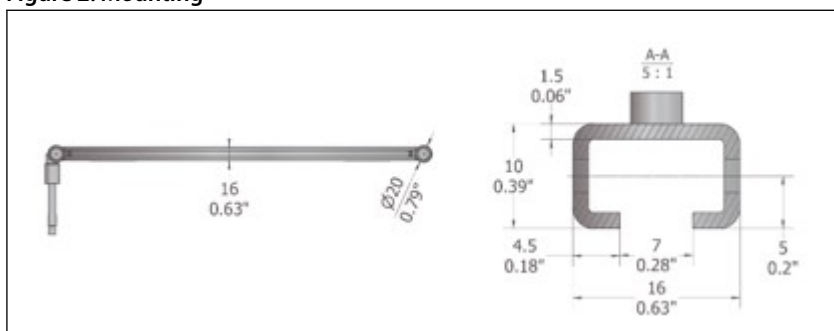
Figure 2: Mounting
