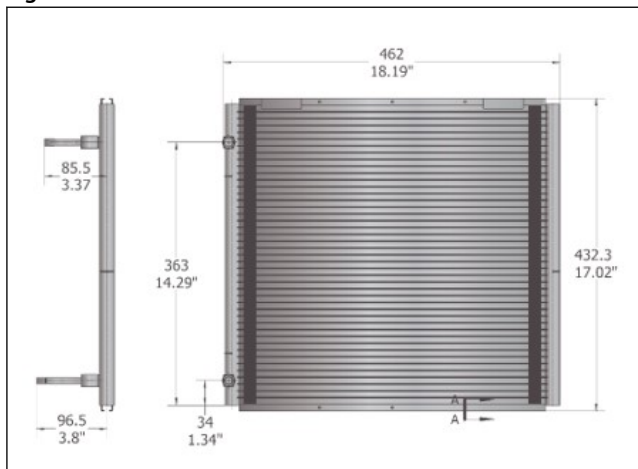
Figure 1: Dimensions
