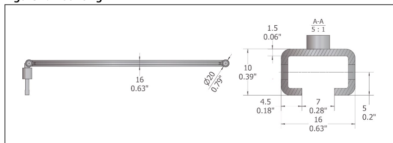
Figure 2: Mounting
