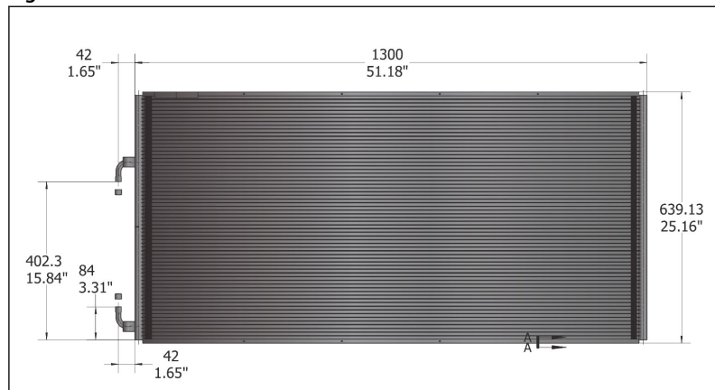
Figure 1: Dimensions
