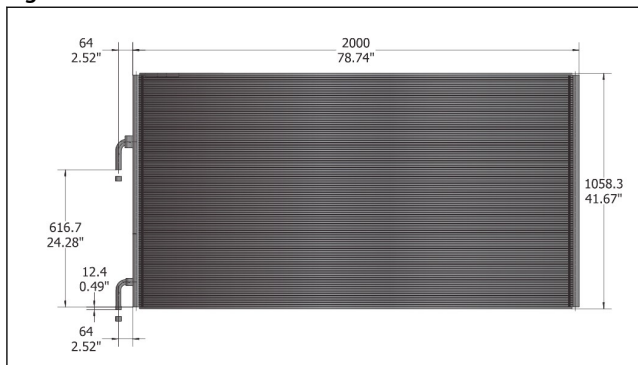
Figure 1: Dimensions
