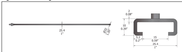
Figure 2: Mounting
